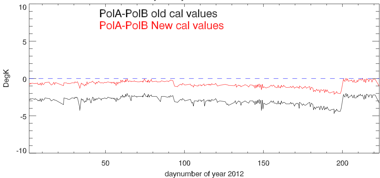
LBW 2012 TsysA-TsysB with old and new cal values
