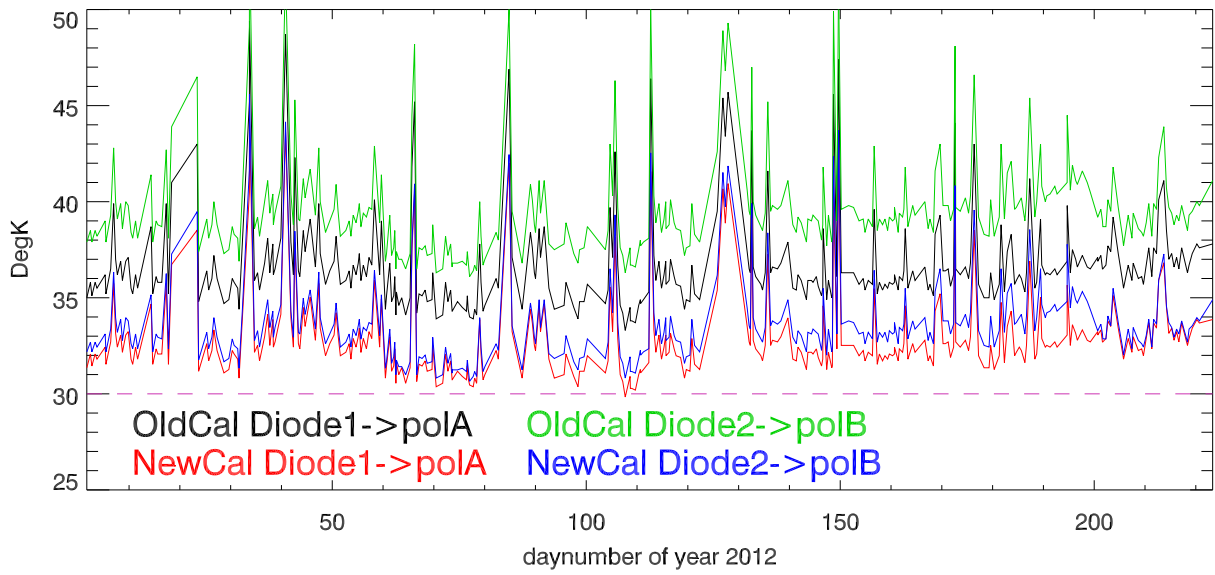
Tsys LBW 2012 Compare old,new cal values. Hcal
