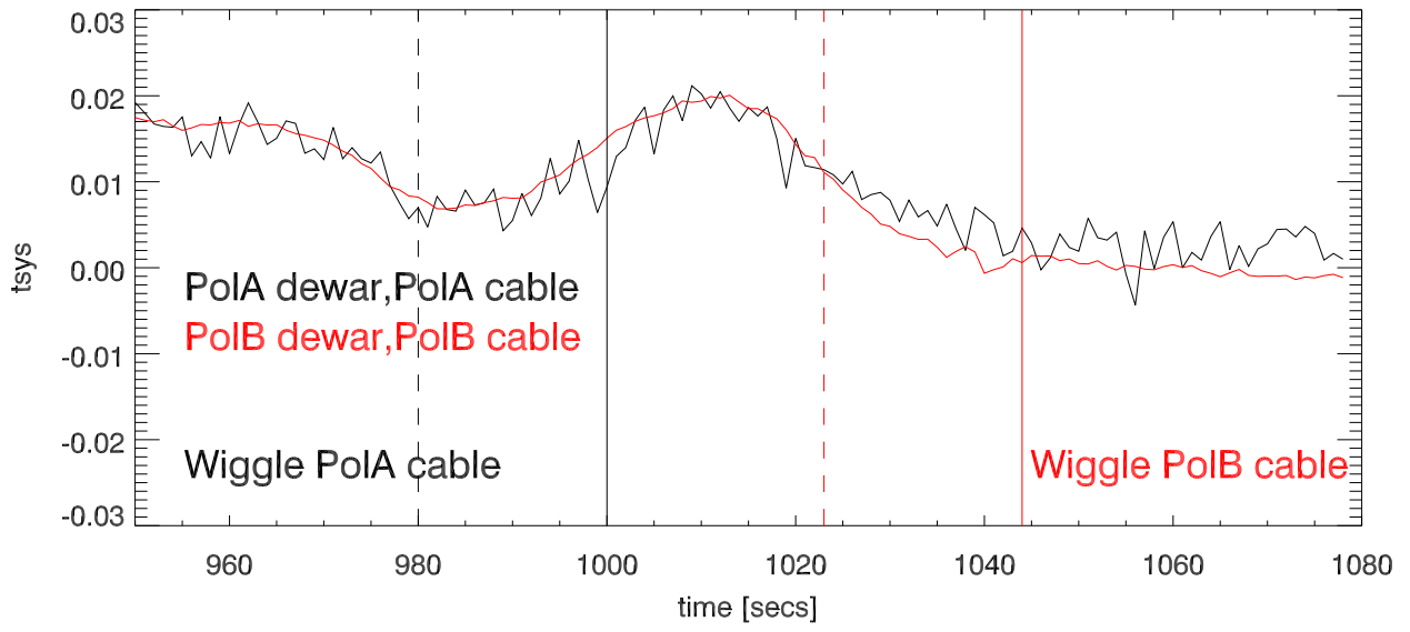
02jul13 xb totPwr vs time. Wiggle rf cables at lo cabinet
