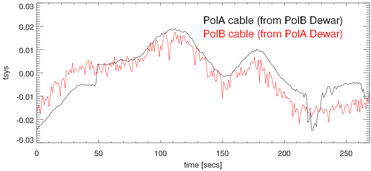
switch poIA,B cables at dewar output
