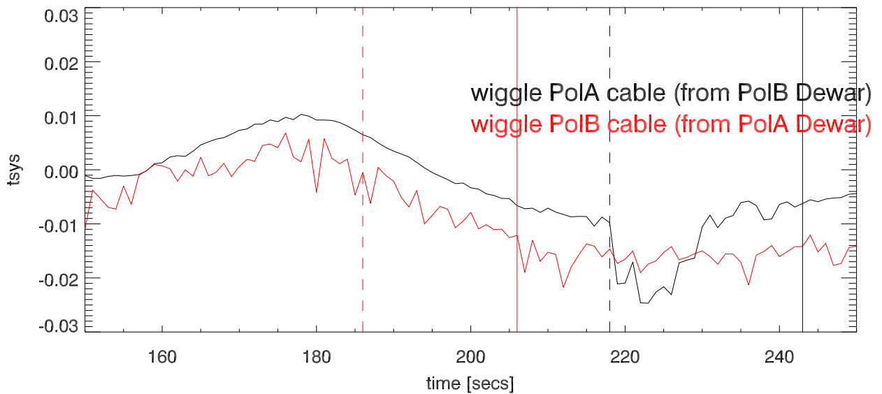
Blowup with poIA,B cables switched at dewar
