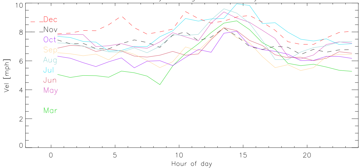
2018 Monthly average wind velocity vs hour
