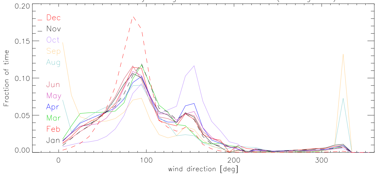
2015 Monthly histogram of wind direction (10 deg bins)
