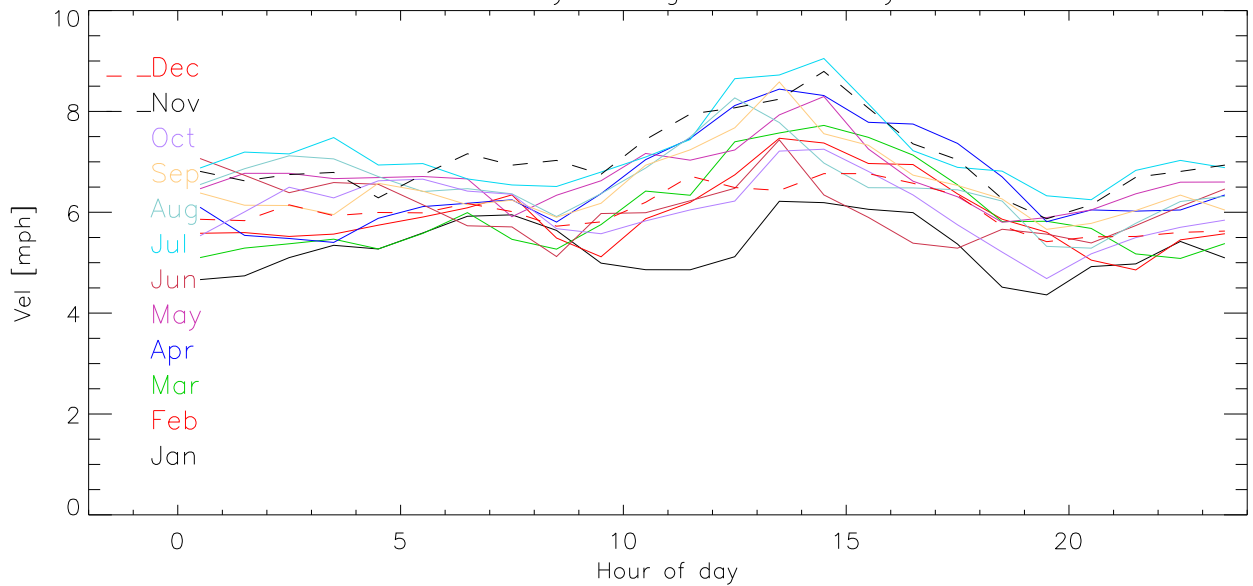
2010 Monthly average wind velocity vs hour
