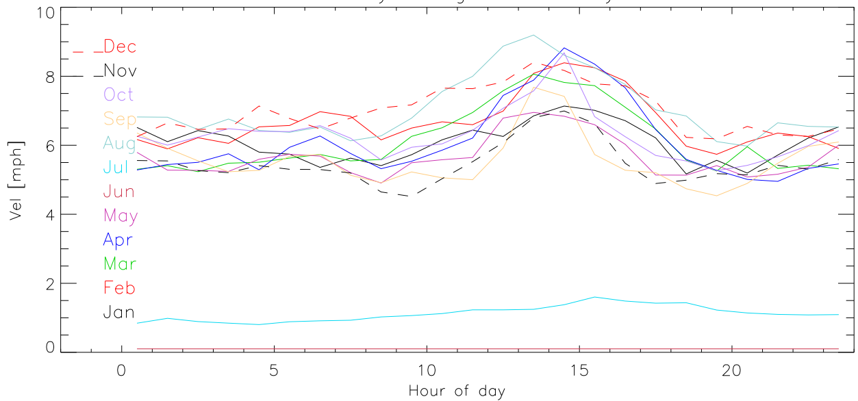
2009 Monthly average wind velocity vs hour
