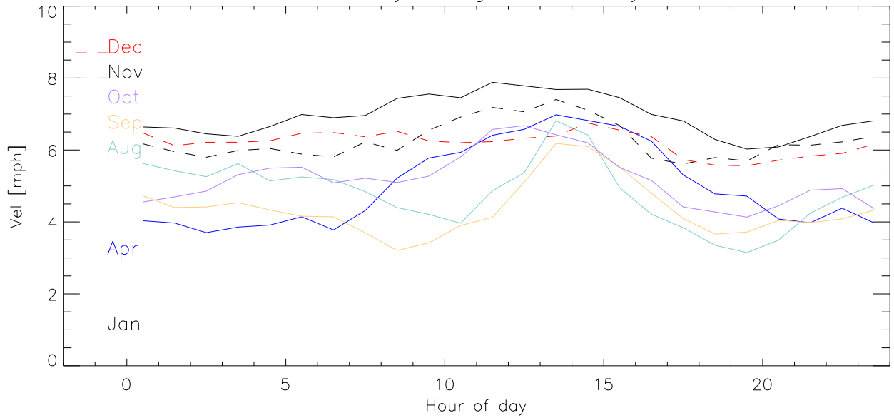
2005 Monthly average wind velocity vs hour
