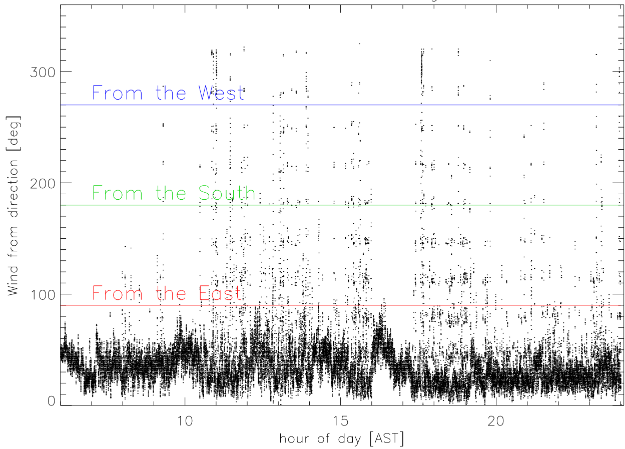
Wind direction for 21aug11
