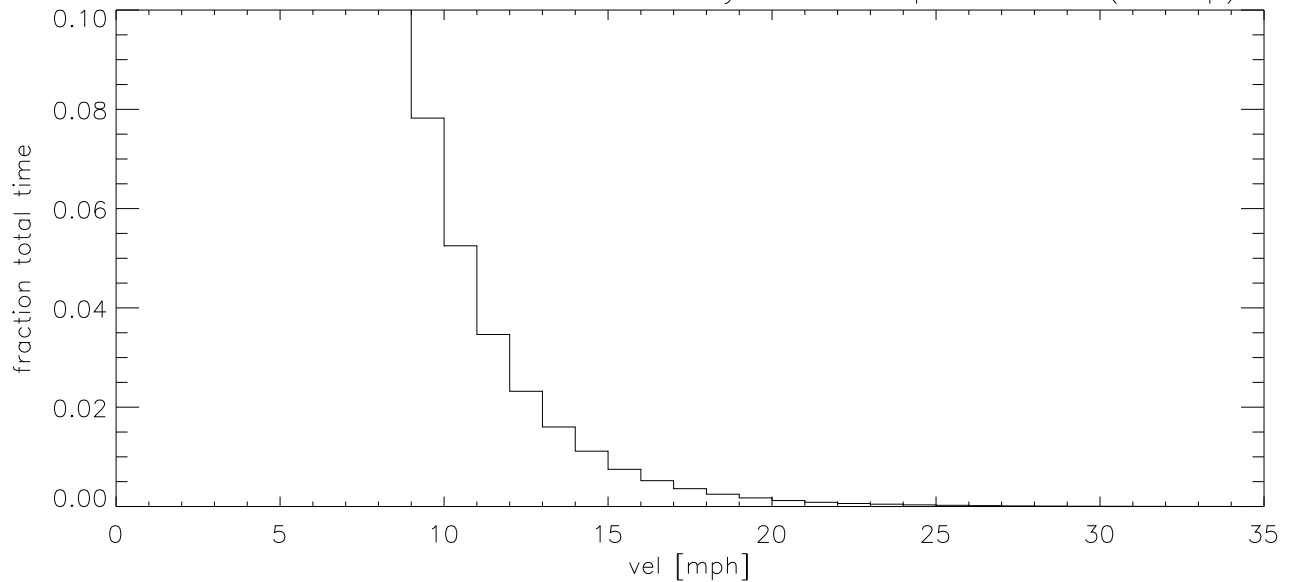
MAY20 Fraction of time wind velocity exceeds specified vel (blowup)
