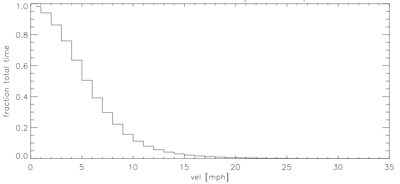
APR20 Fraction of time wind velocity exceeds specified vel (blowup)
