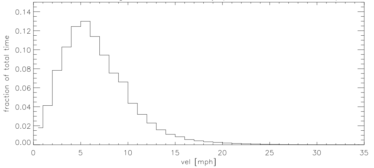
APR20 Fraction of time wind velocity exceeds specified vel
