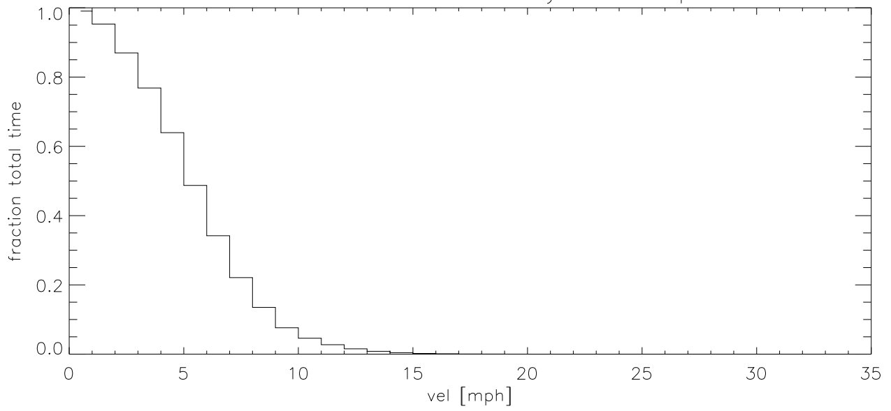
NOV19 Fraction of time wind velocity exceeds specified vel (blowup)
