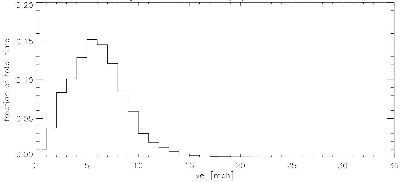
NOV19 Fraction of time wind velocity exceeds specified vel
