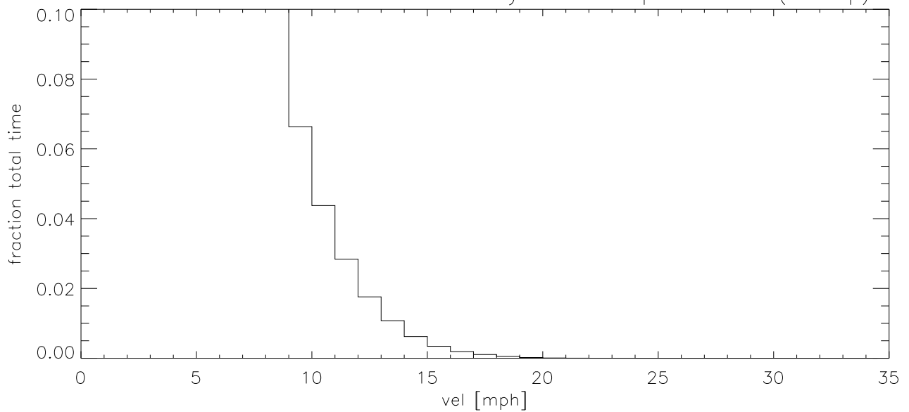
OCT19 Fraction of time wind velocity exceeds specified vel (blowup)
