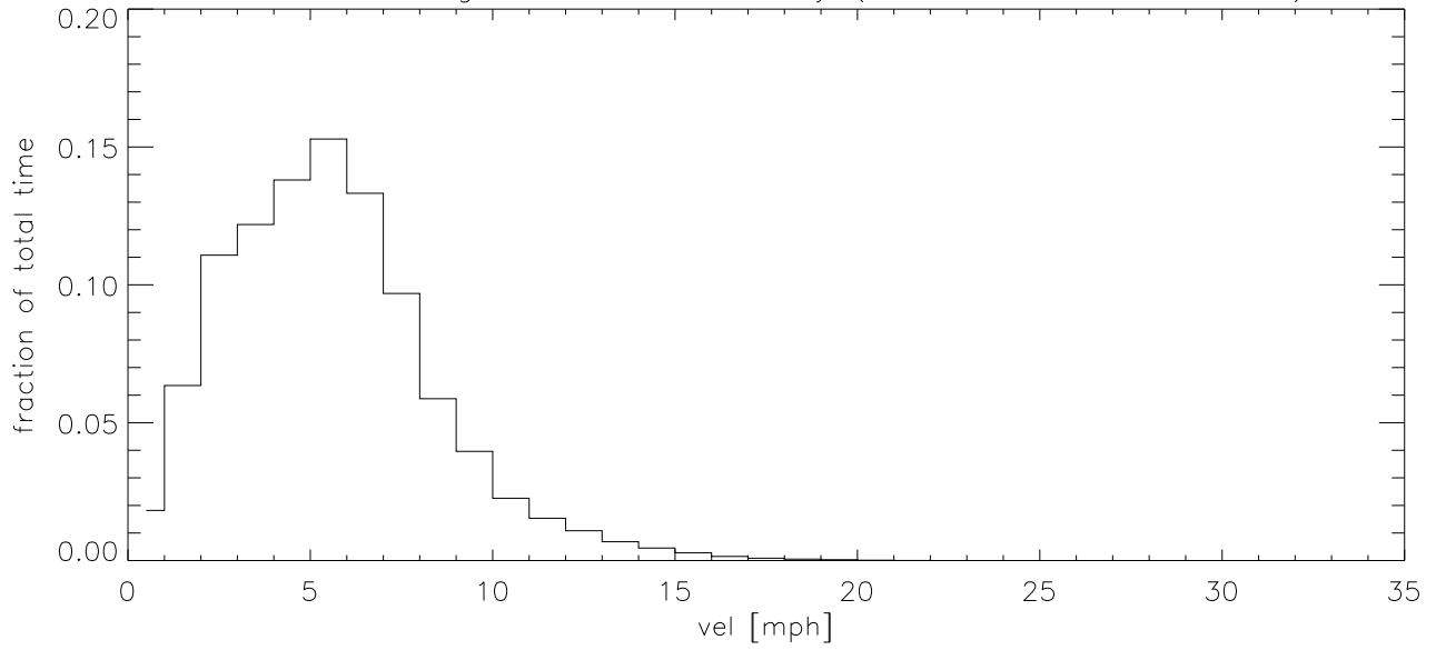
OCT19 Fraction of time wind velocity exceeds specified vel
