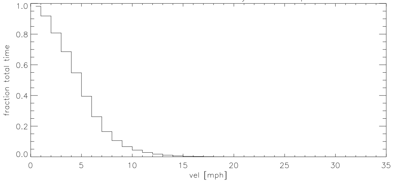
OCT19 Fraction of time wind velocity exceeds specified vel (blowup)
