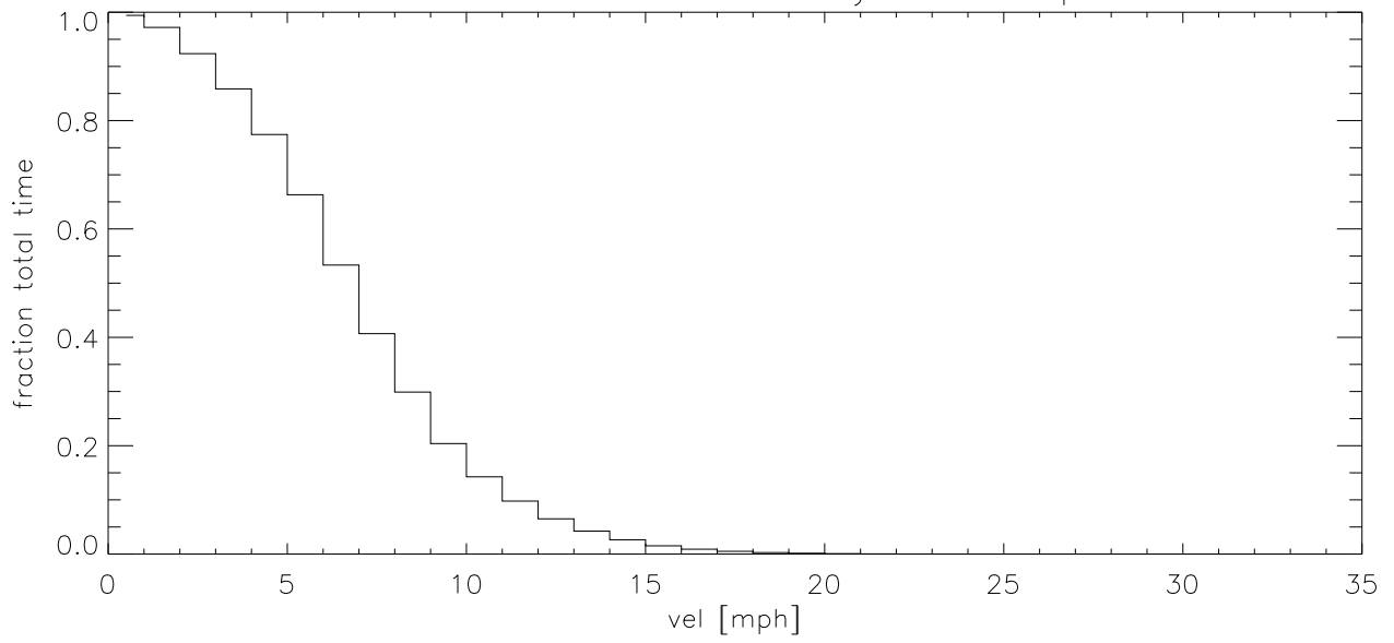
APR19 Fraction of time wind velocity exceeds specified vel (blowup)
