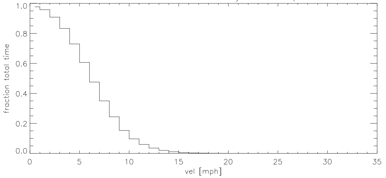
JAN19 Fraction of time wind velocity exceeds specified vel (blowup)
