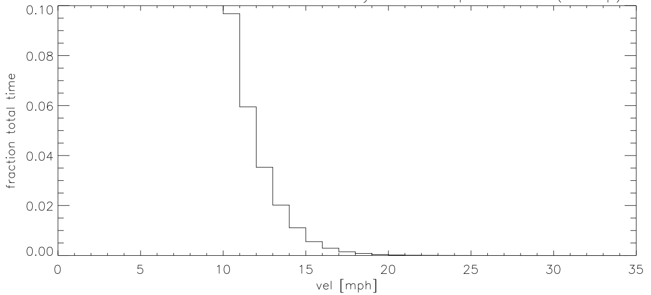
JAN19 Fraction of time wind velocity exceeds specified vel (blowup)
