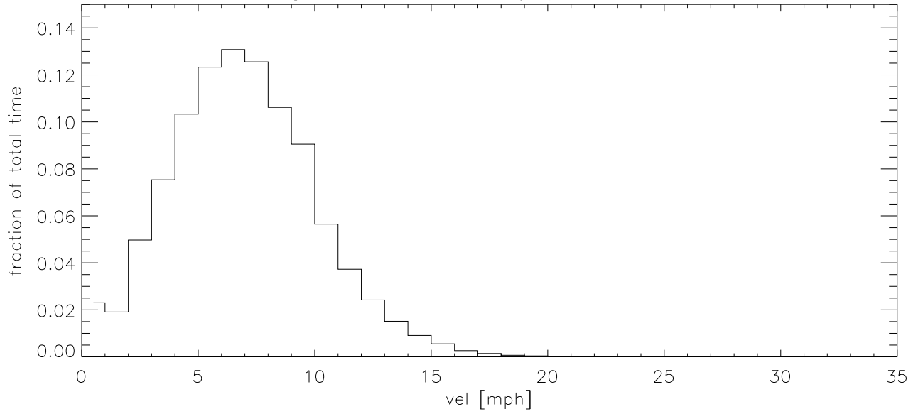
JAN19 Fraction of time wind velocity exceeds specified vel
