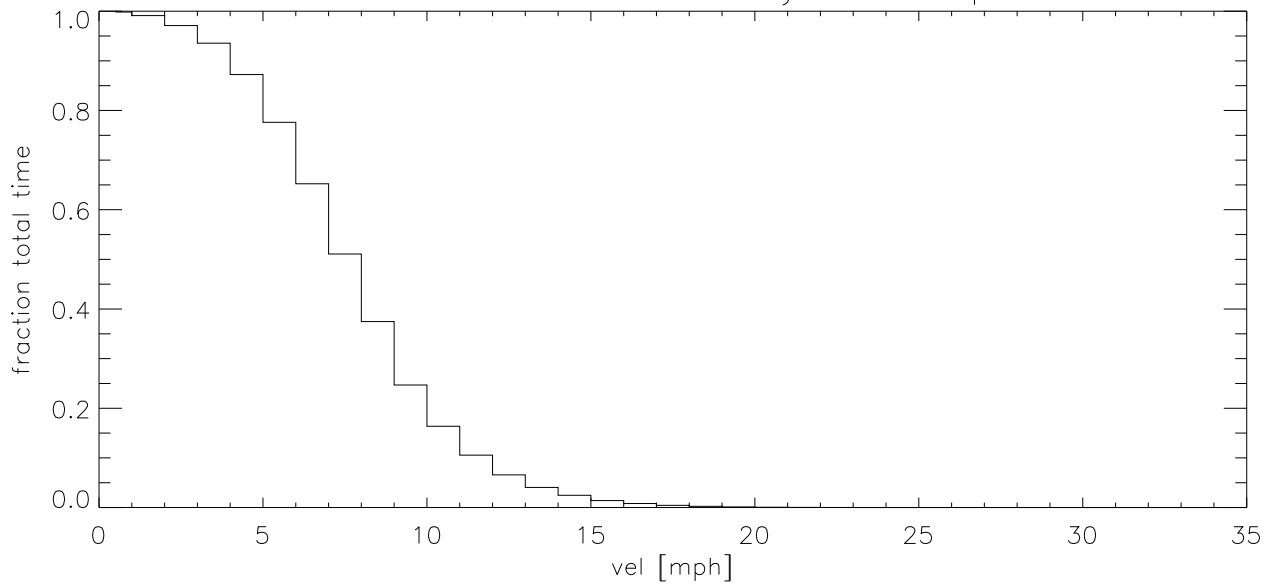
DEC18 Fraction of time wind velocity exceeds specified vel (blowup)
