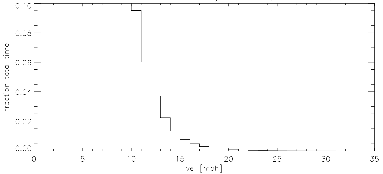
NOV18 Fraction of time wind velocity exceeds specified vel (blowup)
