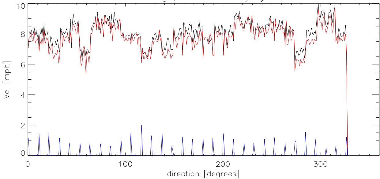
NOV18 Average, median velocity by direction
