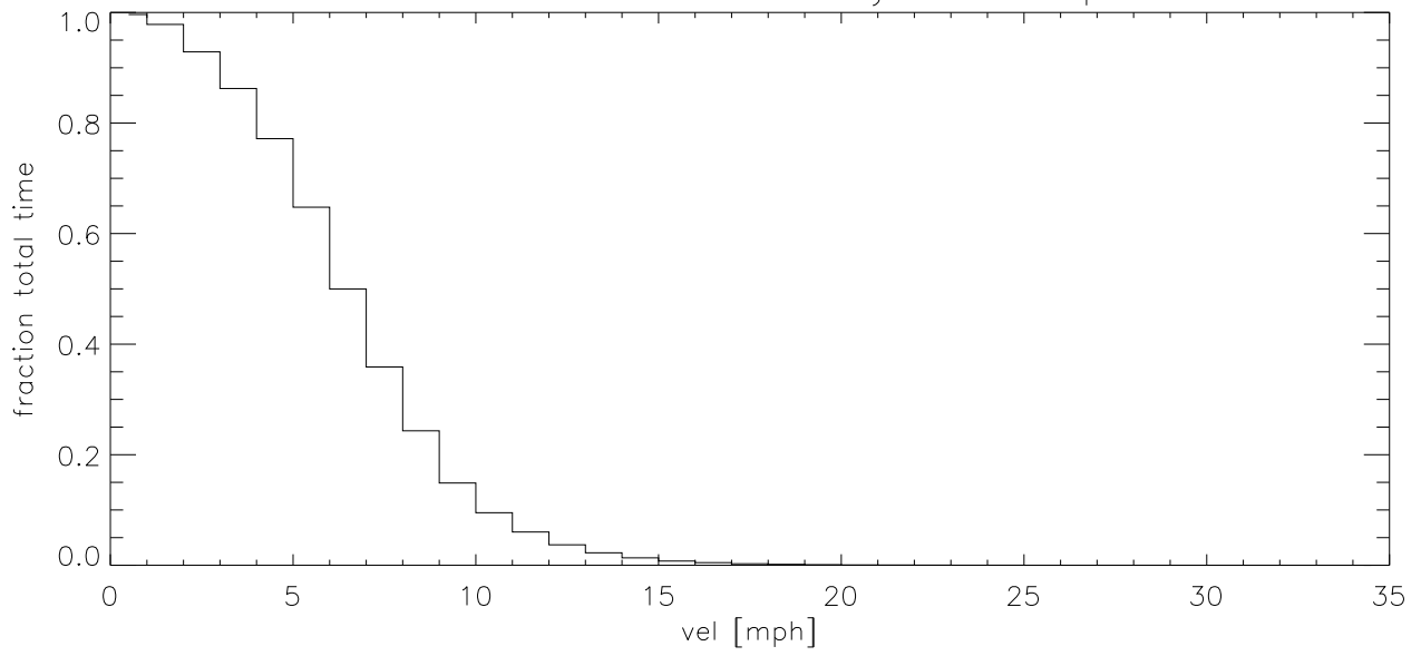
NOV18 Fraction of time wind velocity exceeds specified vel (blowup)
