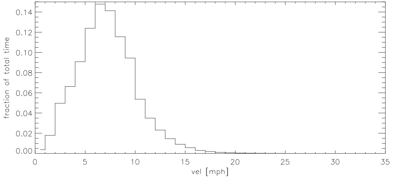
NOV18 Fraction of time wind velocity exceeds specified vel
