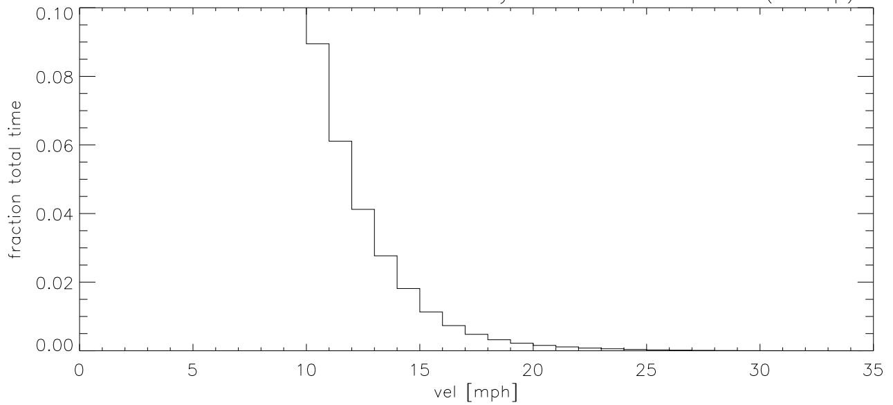
SEP18 Fraction of time wind velocity exceeds specified vel (blowup)
