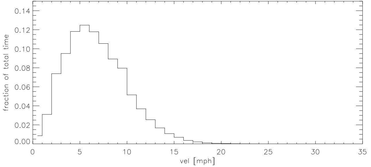
JUN18 Fraction of time wind velocity exceeds specified vel
