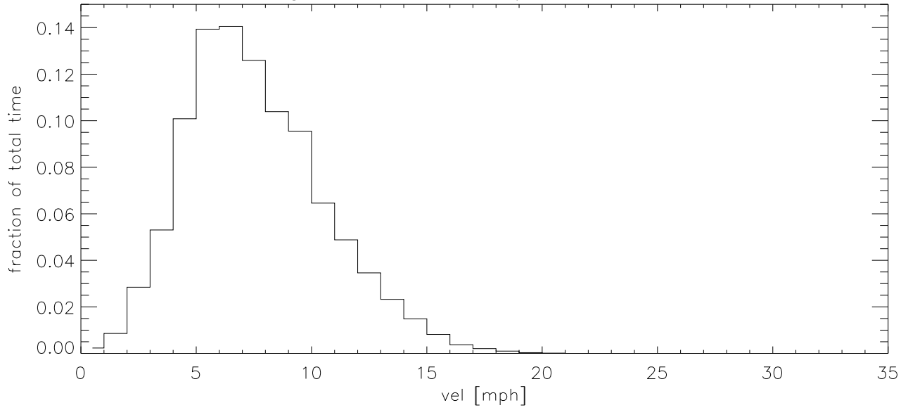
APR18 Fraction of time wind velocity exceeds specified vel
