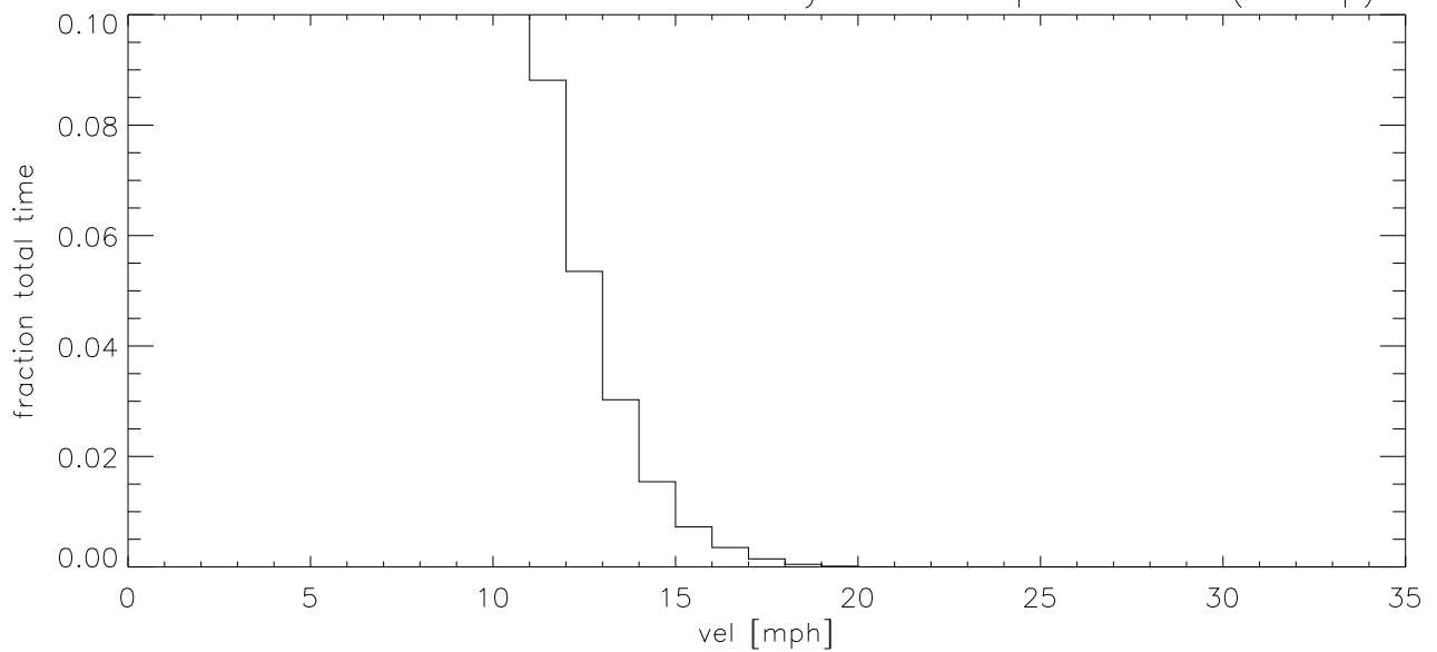
APR18 Fraction of time wind velocity exceeds specified vel (blowup)
