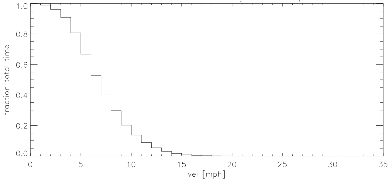
APR18 Fraction of time wind velocity exceeds specified vel (blowup)
