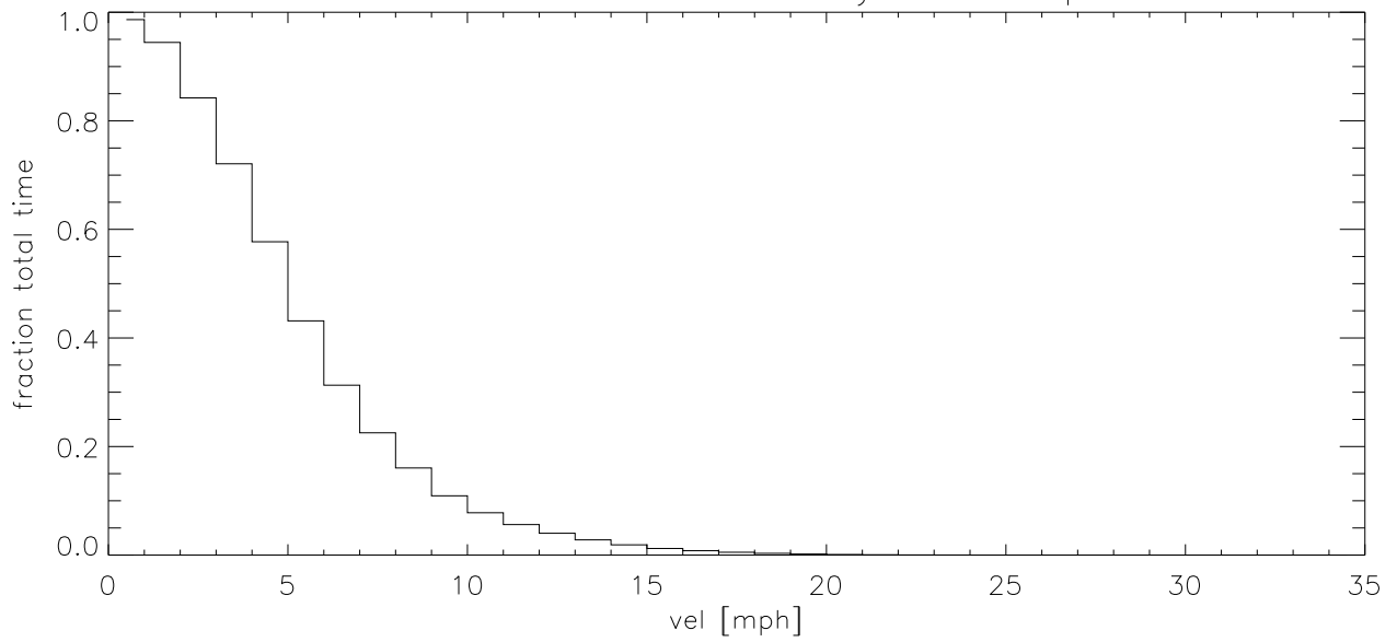
MAR18 Fraction of time wind velocity exceeds specified vel (blowup)
