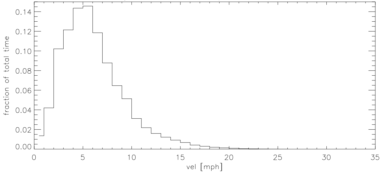
MAR18 Fraction of time wind velocity exceeds specified vel
