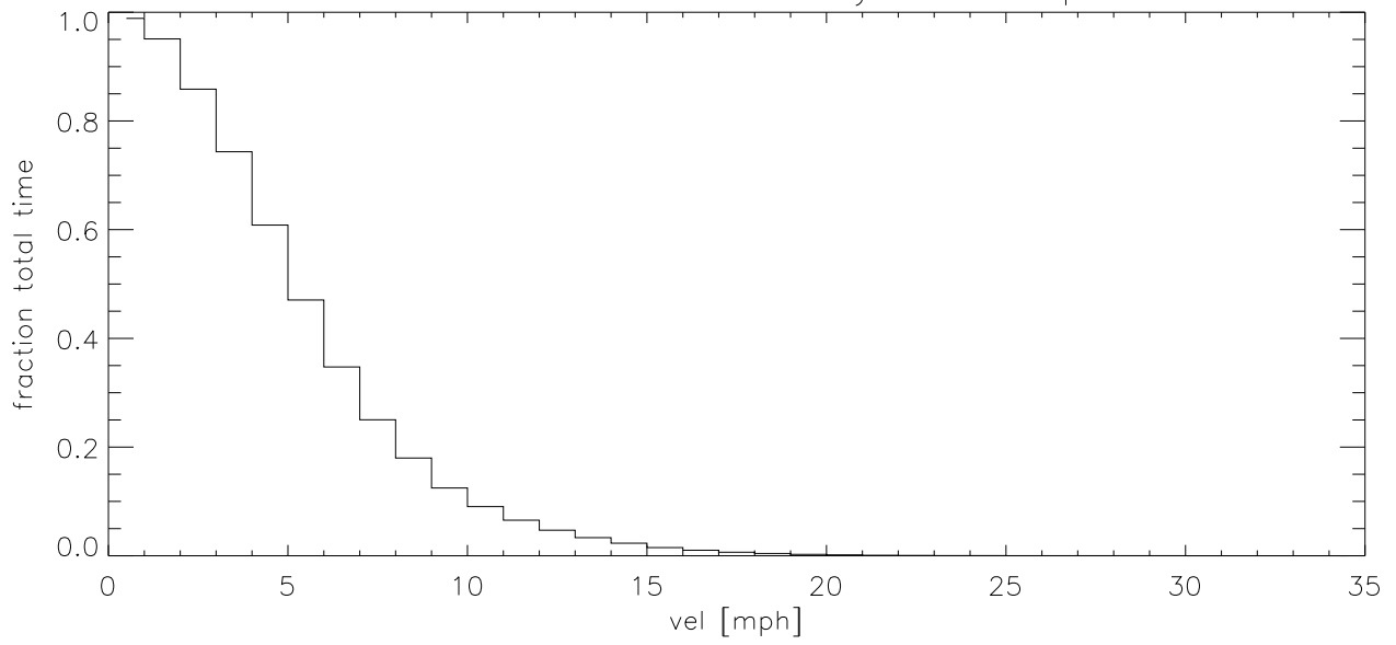
OCT17 Fraction of time wind velocity exceeds specified vel (blowup)
