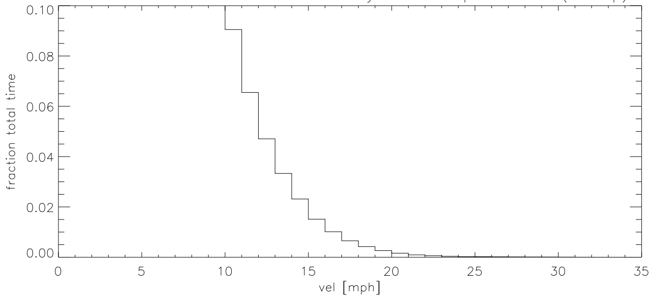
OCT17 Fraction of time wind velocity exceeds specified vel (blowup)
