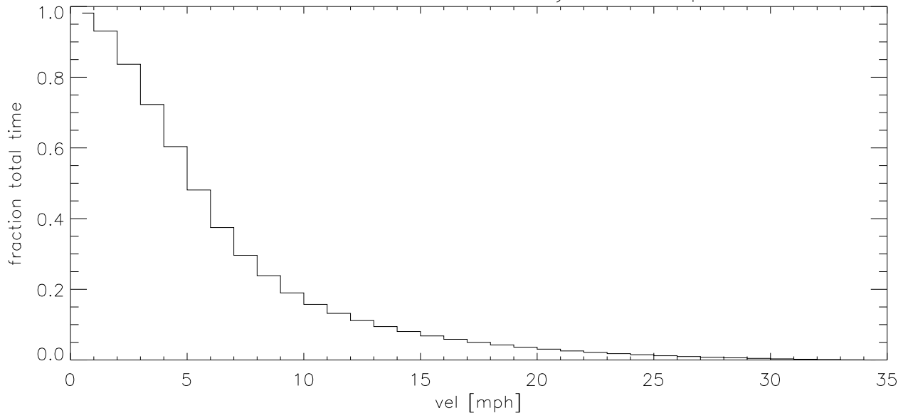
SEP17 Fraction of time wind velocity exceeds specified vel (blowup)
