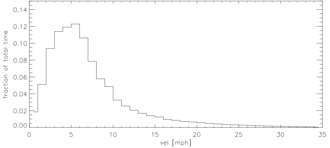
SEP17 Fraction of time wind velocity exceeds specified vel
