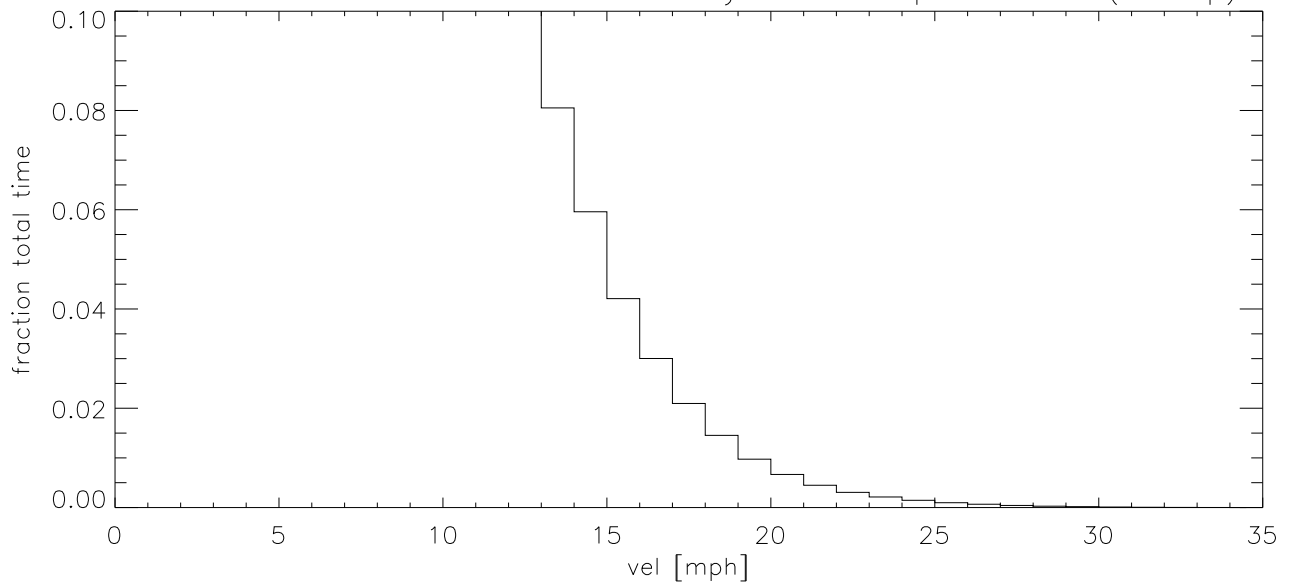
MAR17 Fraction of time wind velocity exceeds specified vel (blowup)
