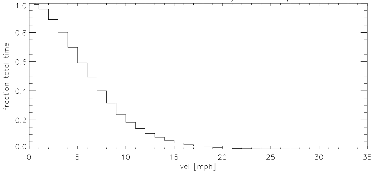
MAR17 Fraction of time wind velocity exceeds specified vel (blowup)
