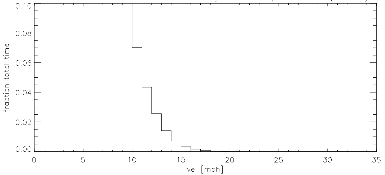
FEB17 Fraction of time wind velocity exceeds specified vel (blowup)
