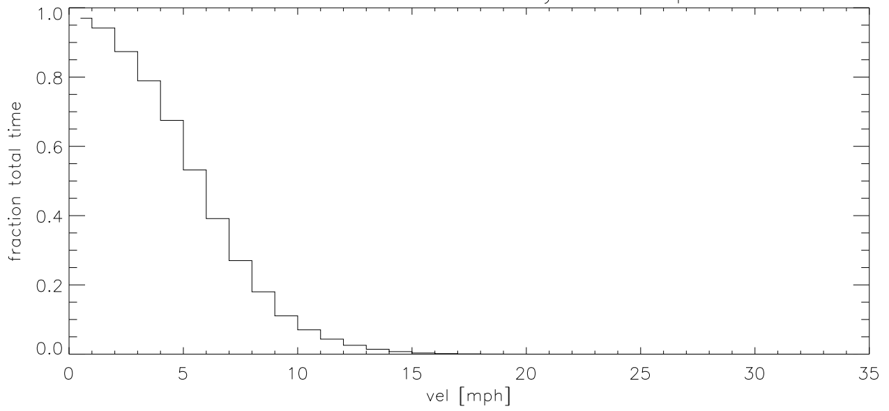
FEB17 Fraction of time wind velocity exceeds specified vel (blowup)
