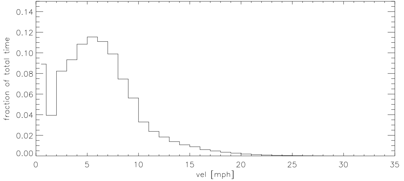
OCT16 Fraction of time wind velocity exceeds specified vel
