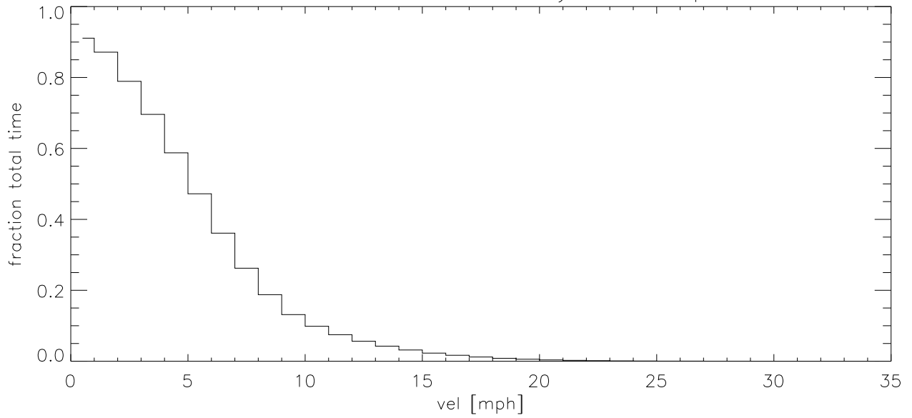
OCT16 Fraction of time wind velocity exceeds specified vel (blowup)
