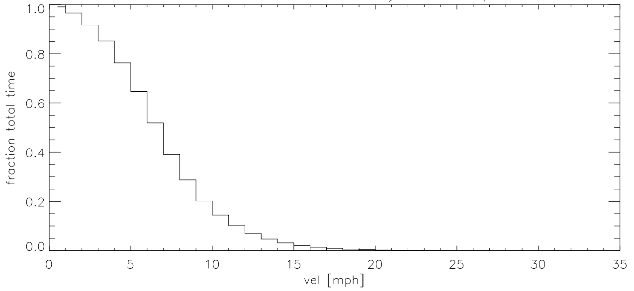
SEP16 Fraction of time wind velocity exceeds specified vel (blowup)
