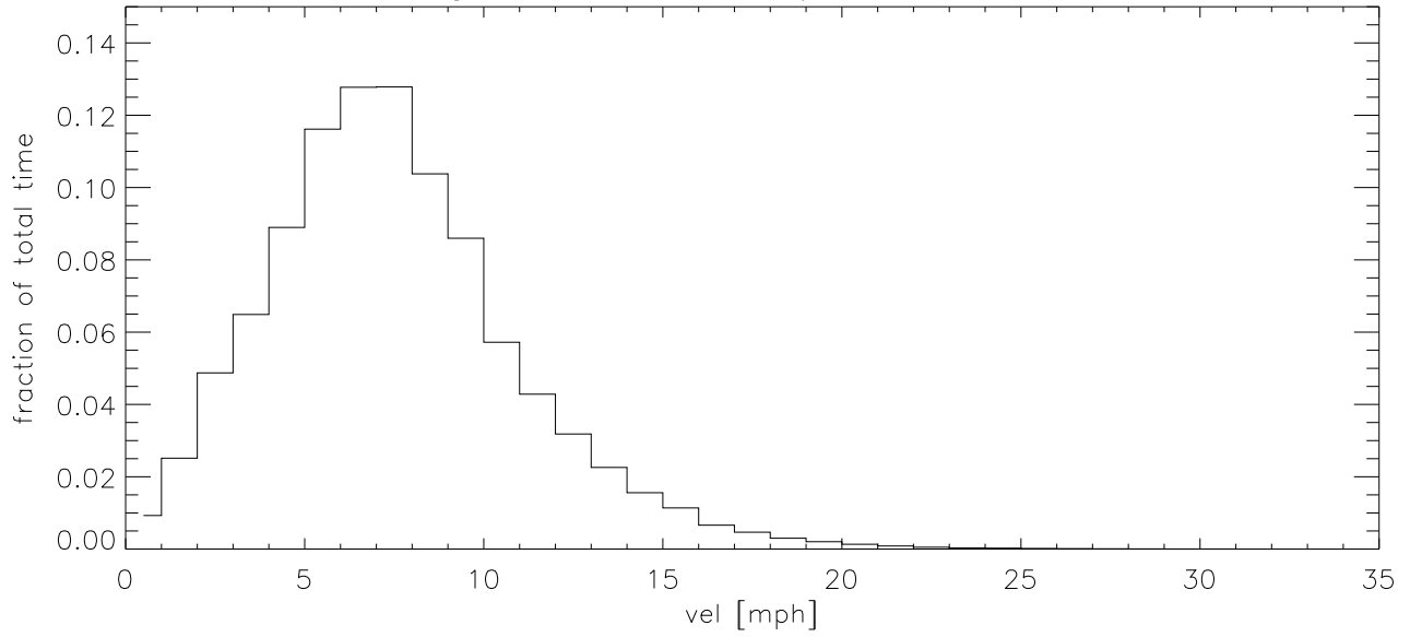
SEP16 Fraction of time wind velocity exceeds specified vel
