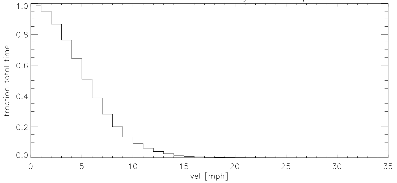
AUG16 Fraction of time wind velocity exceeds specified vel (blowup)
