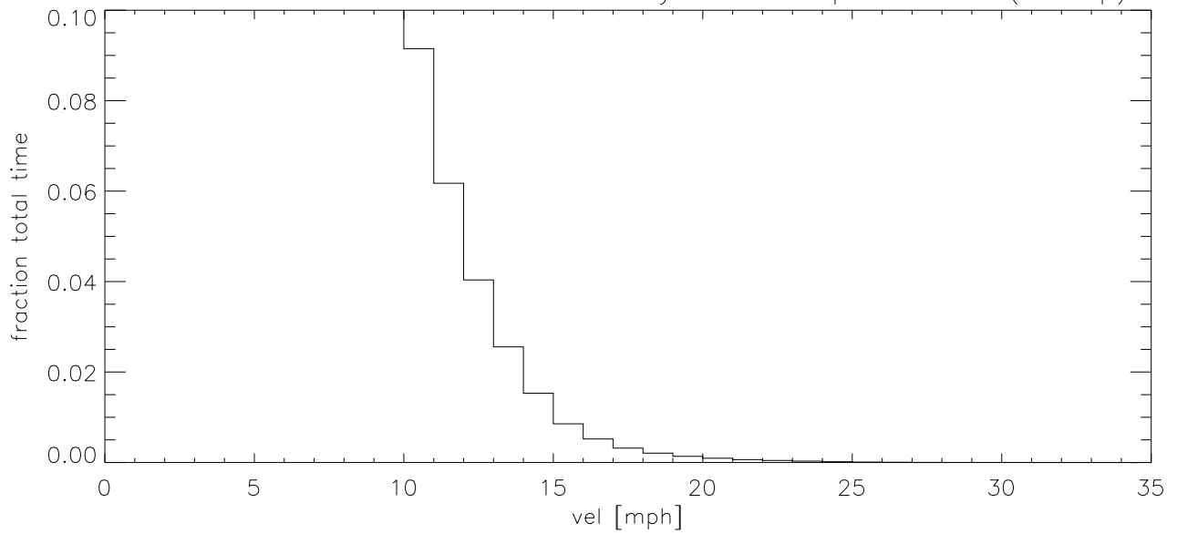
AUG16 Fraction of time wind velocity exceeds specified vel (blowup)
