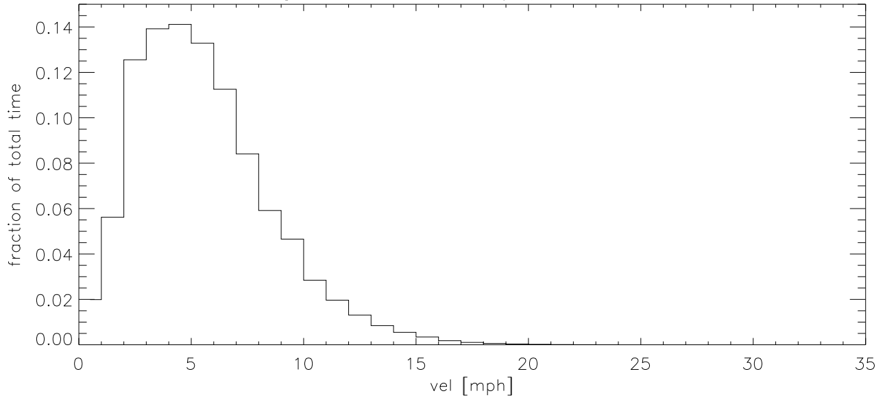
APR16 Fraction of time wind velocity exceeds specified vel
