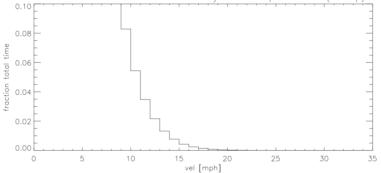
APR16 Fraction of time wind velocity exceeds specified vel (blowup)
