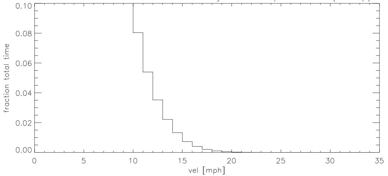
FEB16 Fraction of time wind velocity exceeds specified vel (blowup)
