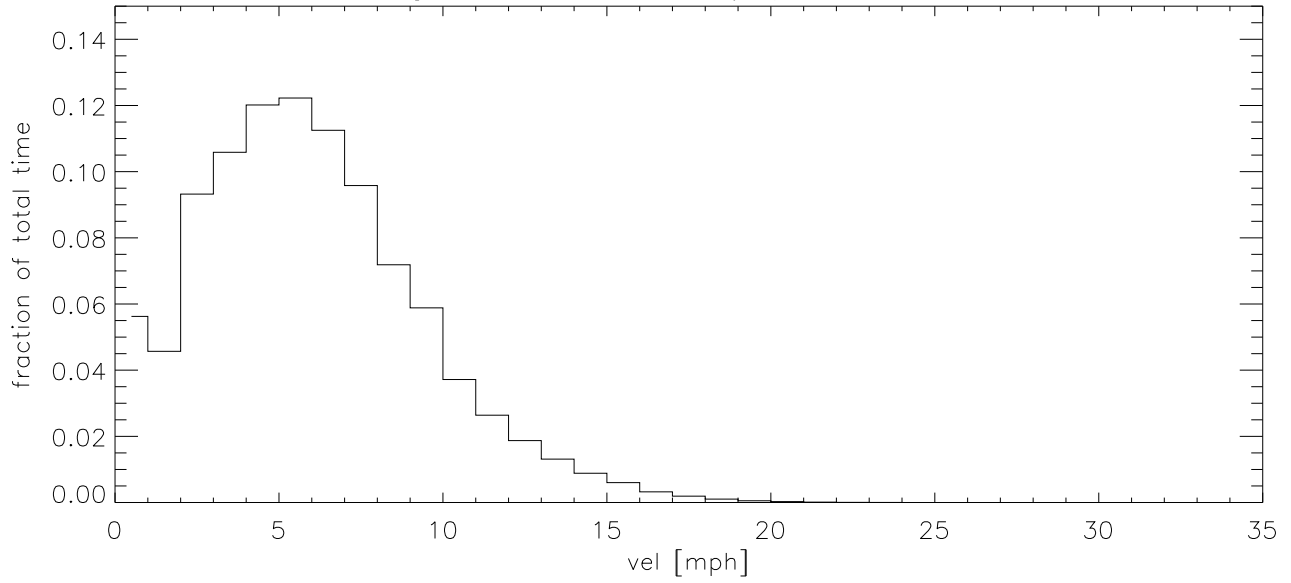
FEB16 Fraction of time wind velocity exceeds specified vel
