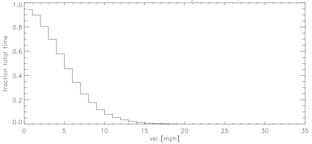
FEB16 Fraction of time wind velocity exceeds specified vel (blowup)
