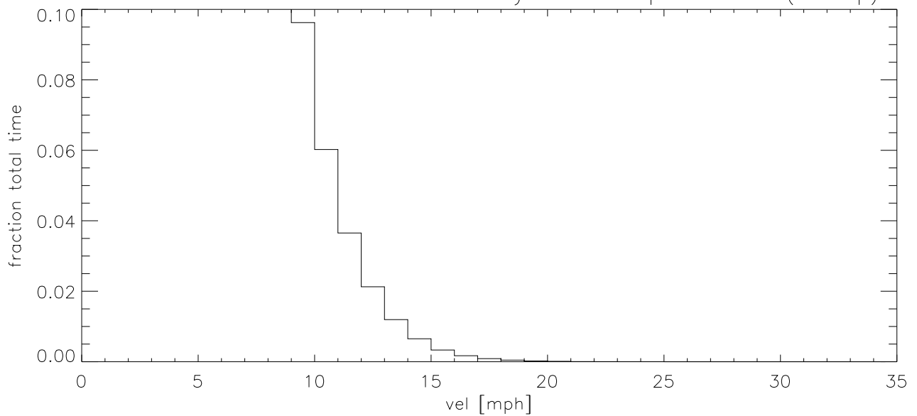
NOV15 Fraction of time wind velocity exceeds specified vel (blowup)
