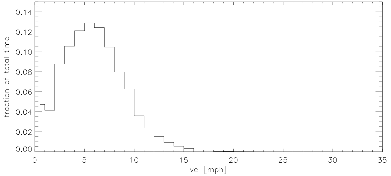
NOV15 Fraction of time wind velocity exceeds specified vel
