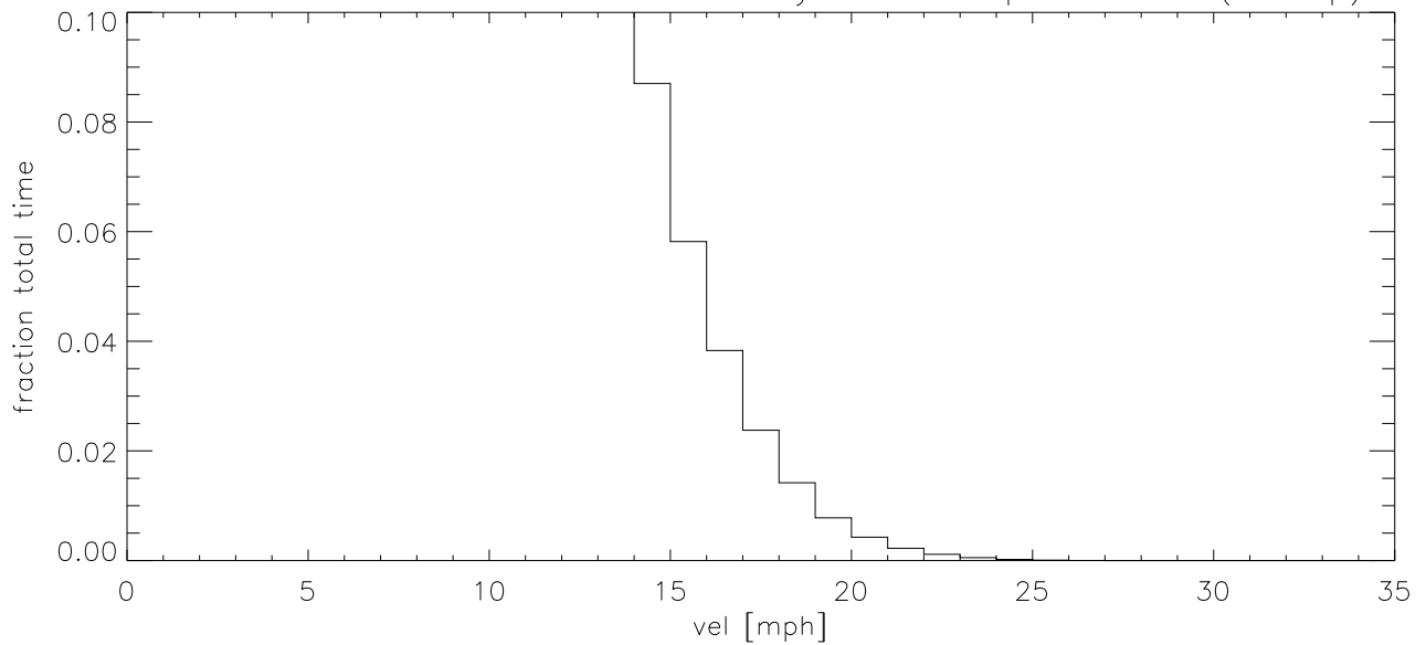
JUL15 Fraction of time wind velocity exceeds specified vel (blowup)
