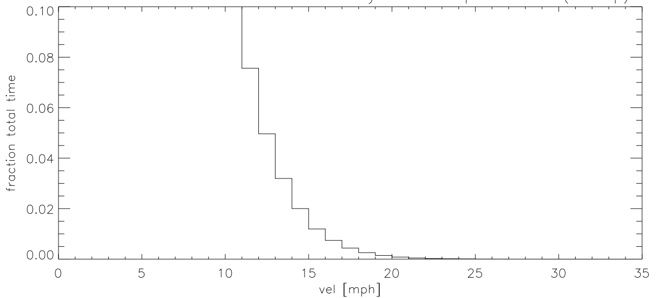
MAR15 Fraction of time wind velocity exceeds specified vel (blowup)
