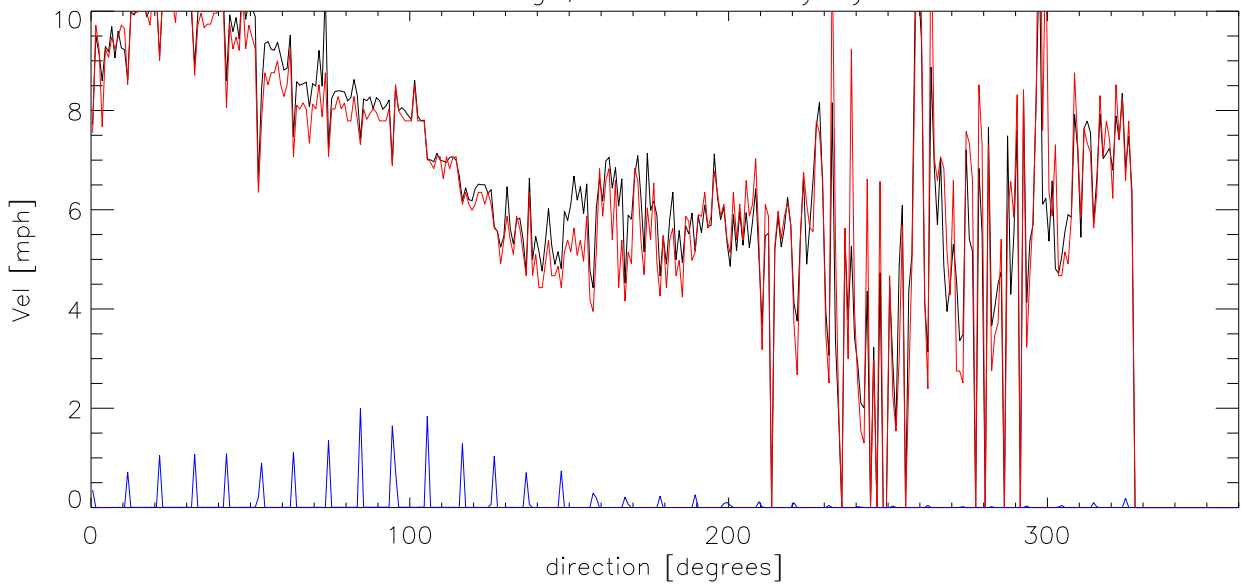
MAR15 Average, median velocity by direction
