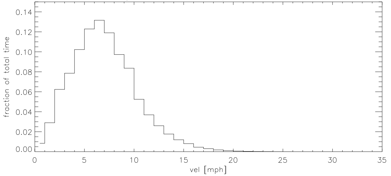
MAR15 Fraction of time wind velocity exceeds specified vel
