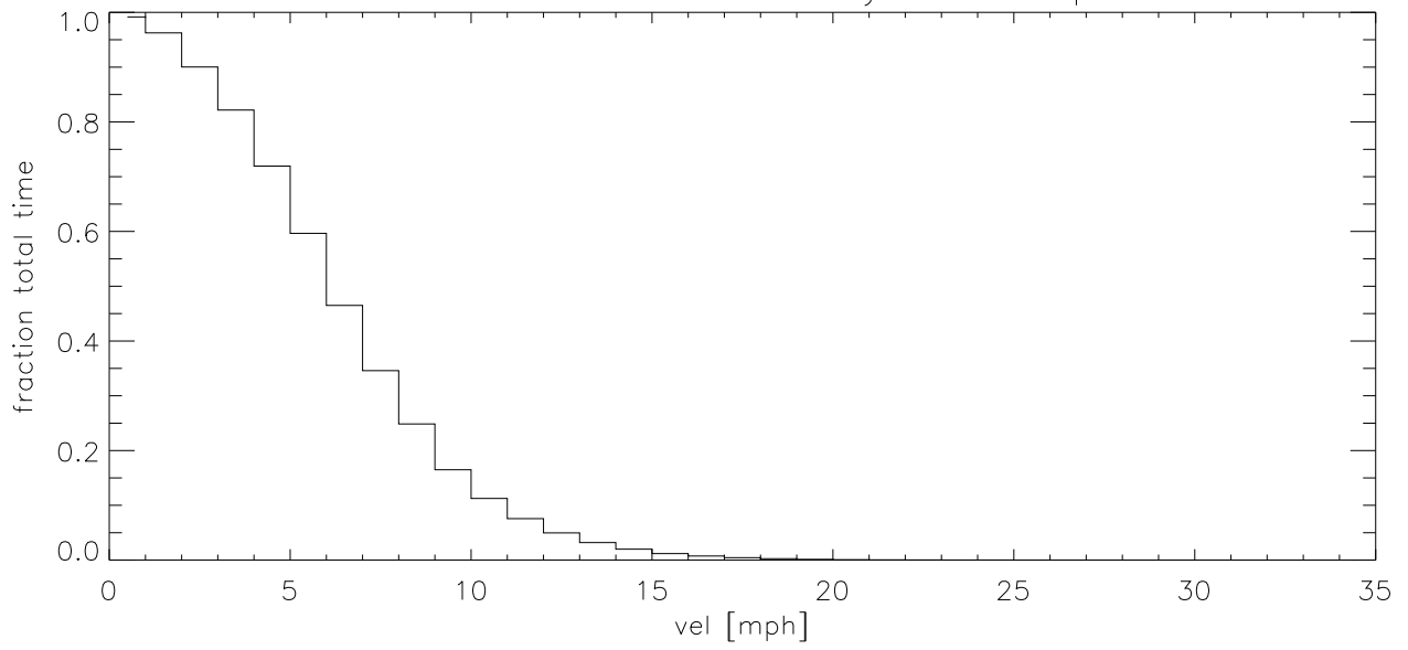
MAR15 Fraction of time wind velocity exceeds specified vel (blowup)
