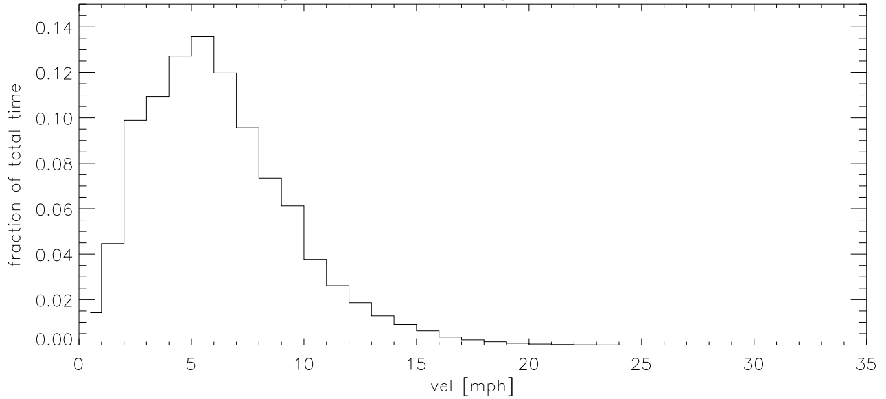
JUL14 Fraction of time wind velocity exceeds specified vel
