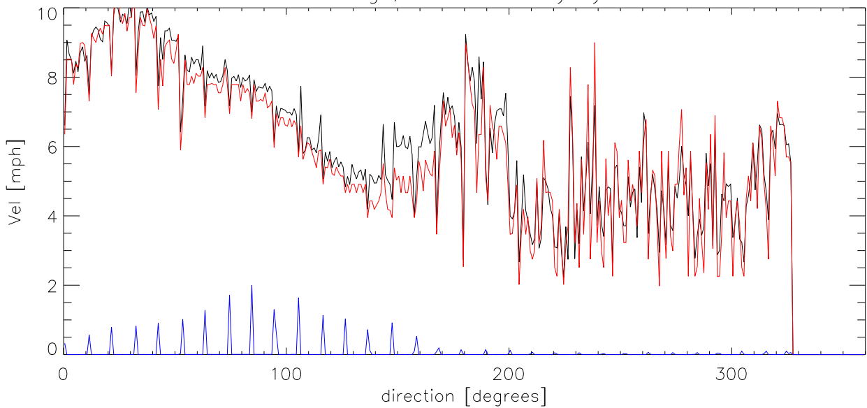
JUL14 Average, median velocity by direction
