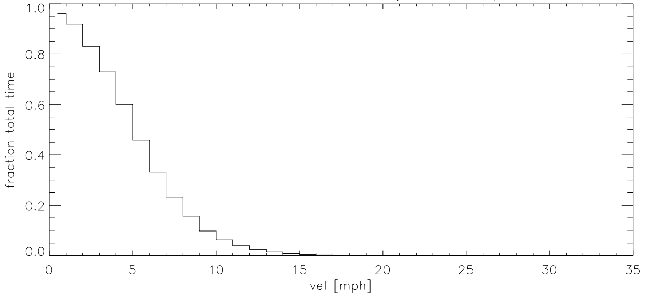
JUN14 Fraction of time wind velocity exceeds specified vel (blowup)
