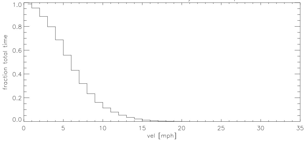
APR14 Fraction of time wind velocity exceeds specified vel (blowup)
