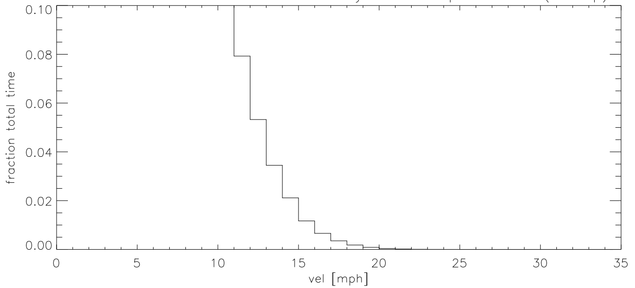
APR14 Fraction of time wind velocity exceeds specified vel (blowup)
