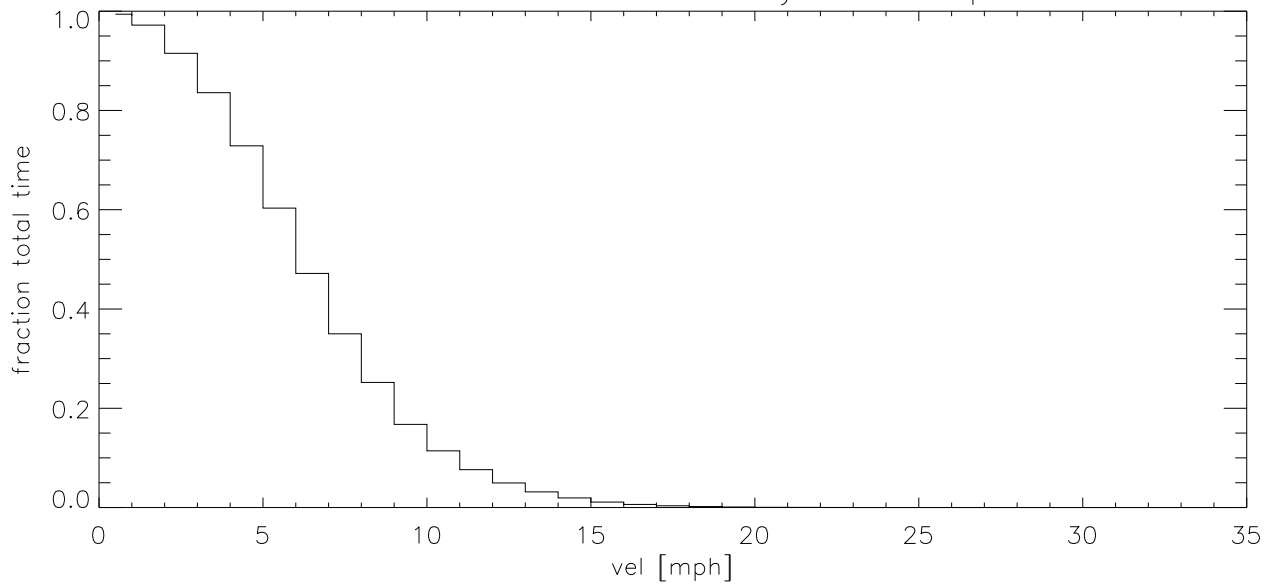
FEB14 Fraction of time wind velocity exceeds specified vel (blowup)
