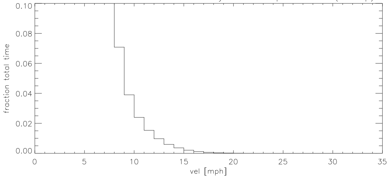
OCT13 Fraction of time wind velocity exceeds specified vel (blowup)
