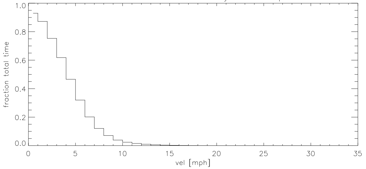
OCT13 Fraction of time wind velocity exceeds specified vel (blowup)
