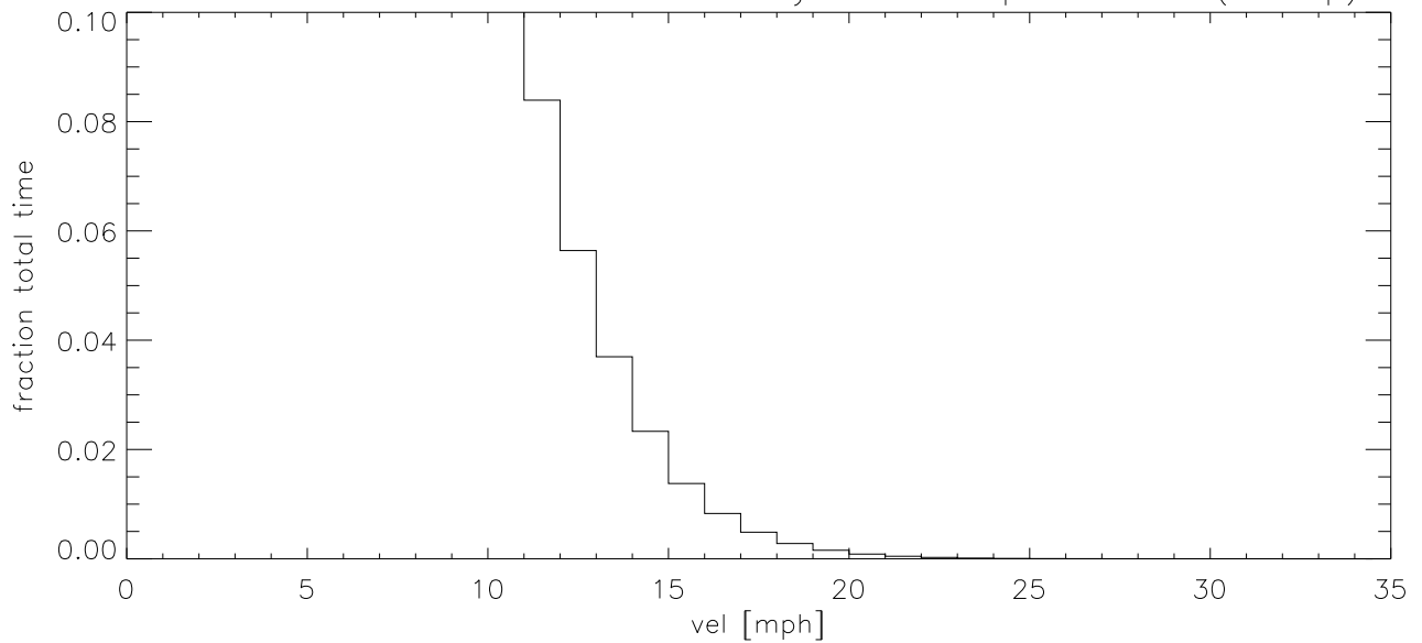
JUL13 Fraction of time wind velocity exceeds specified vel (blowup)
