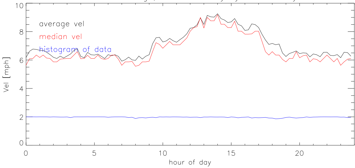
JUL13 Average, median velocity by direction
