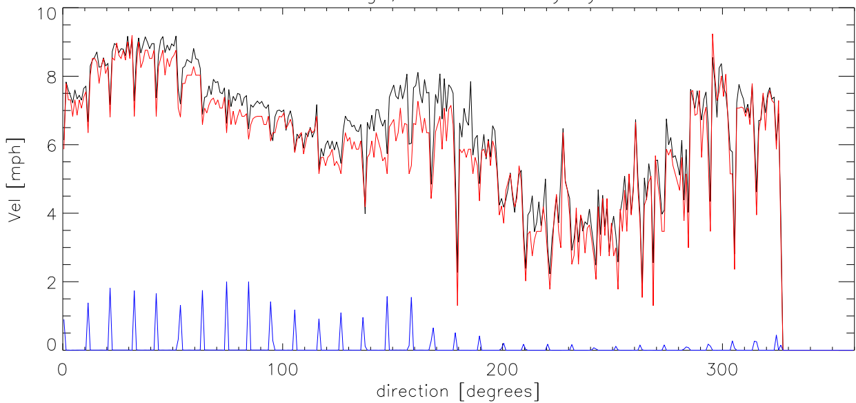
MAR13 Average, median velocity by direction
