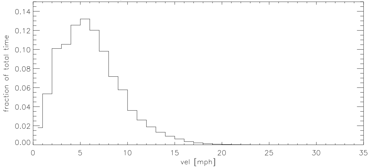
MAR13 Fraction of time wind velocity exceeds specified vel
