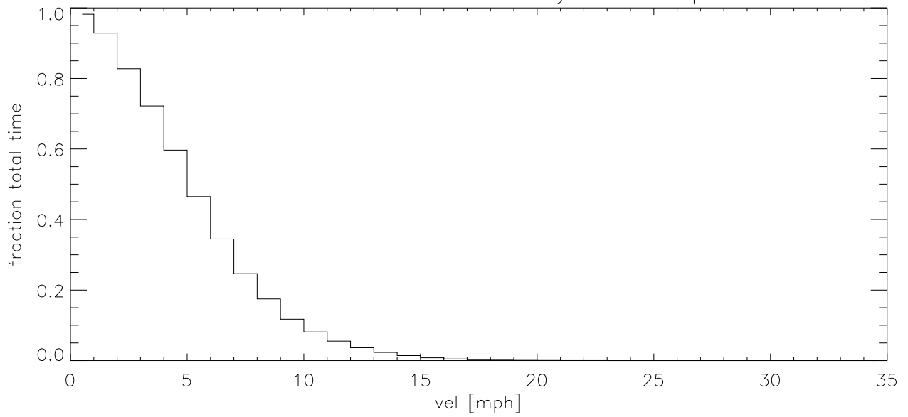
MAR13 Fraction of time wind velocity exceeds specified vel (blowup)
