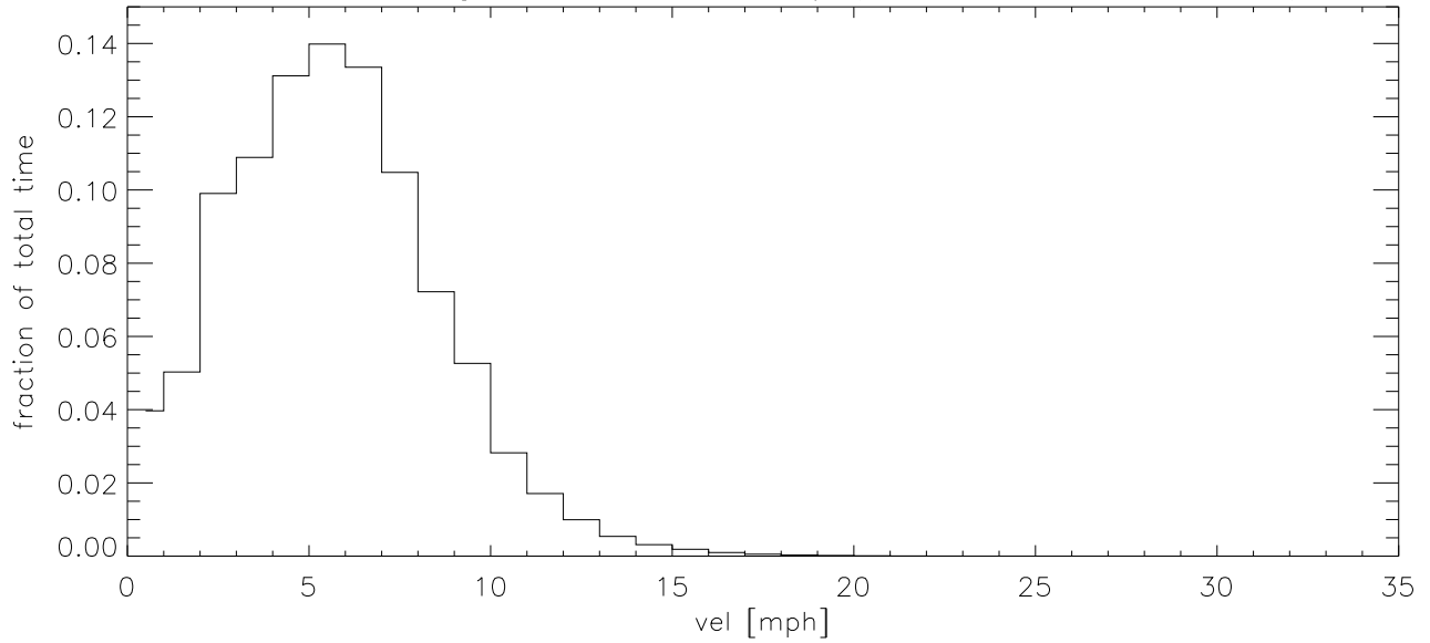
NOV12 Fraction of time wind velocity exceeds specified vel
