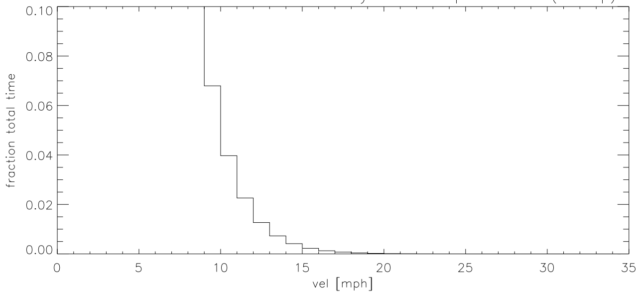
NOV12 Fraction of time wind velocity exceeds specified vel (blowup)
