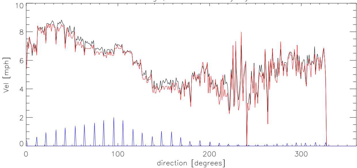
NOV12 Average, median velocity by direction
