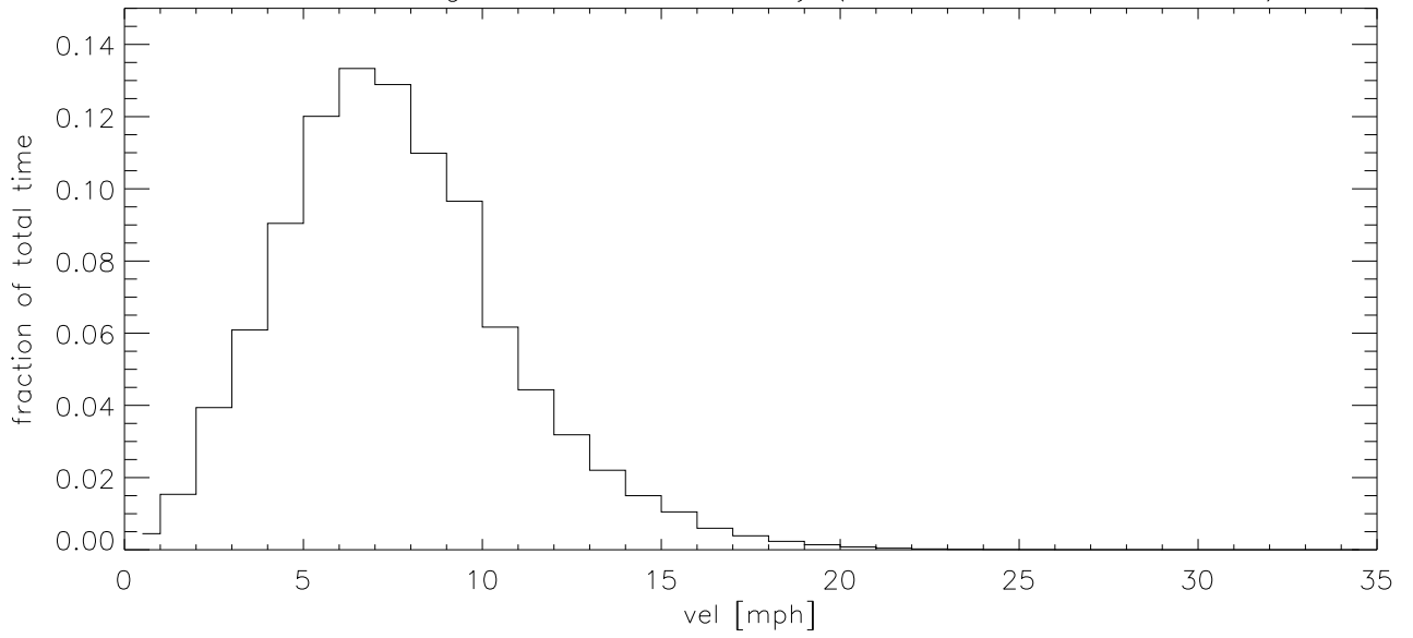
JUL12 Fraction of time wind velocity exceeds specified vel
