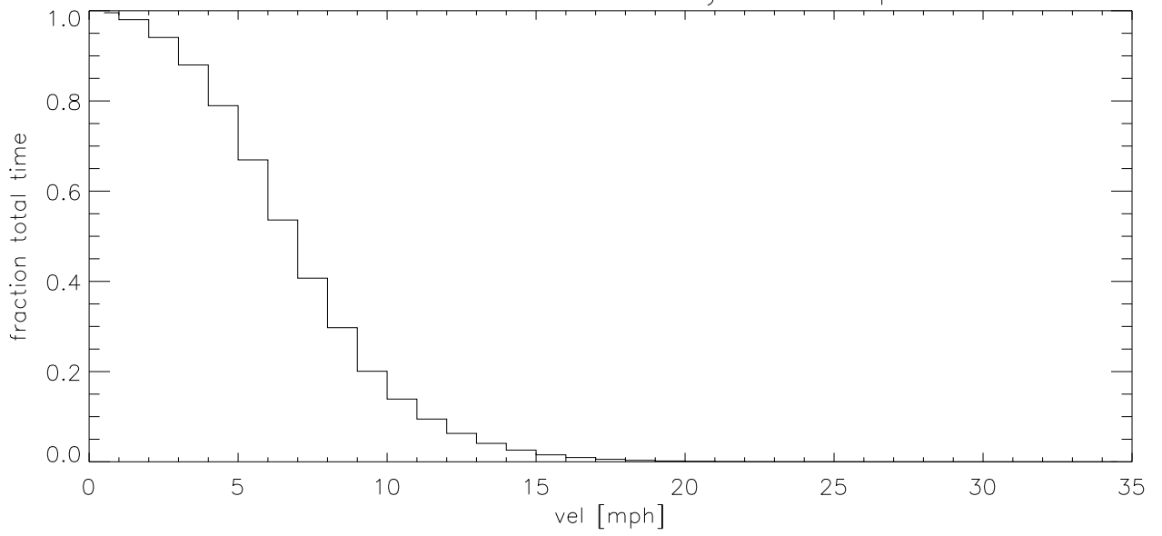
JUL12 Fraction of time wind velocity exceeds specified vel (blowup)
