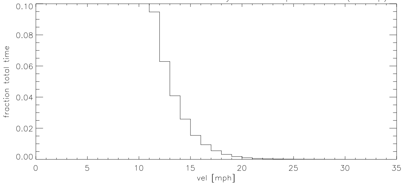
JUL12 Fraction of time wind velocity exceeds specified vel (blowup)
