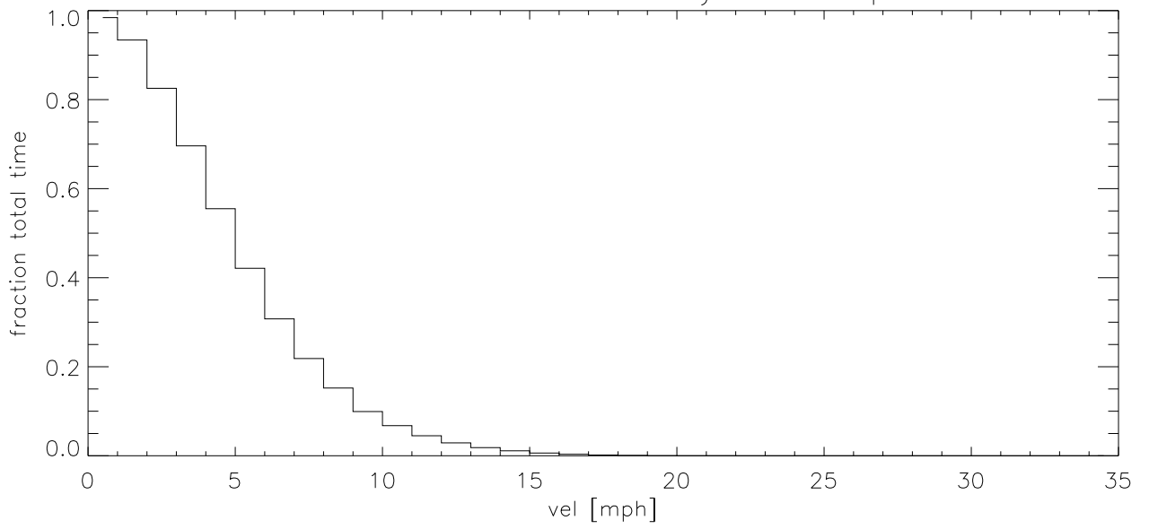
JUN12 Fraction of time wind velocity exceeds specified vel (blowup)
