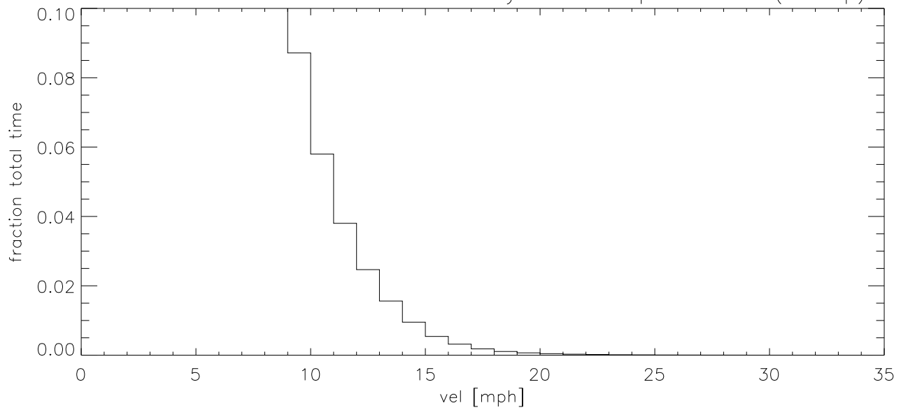
MAY12 Fraction of time wind velocity exceeds specified vel (blowup)
