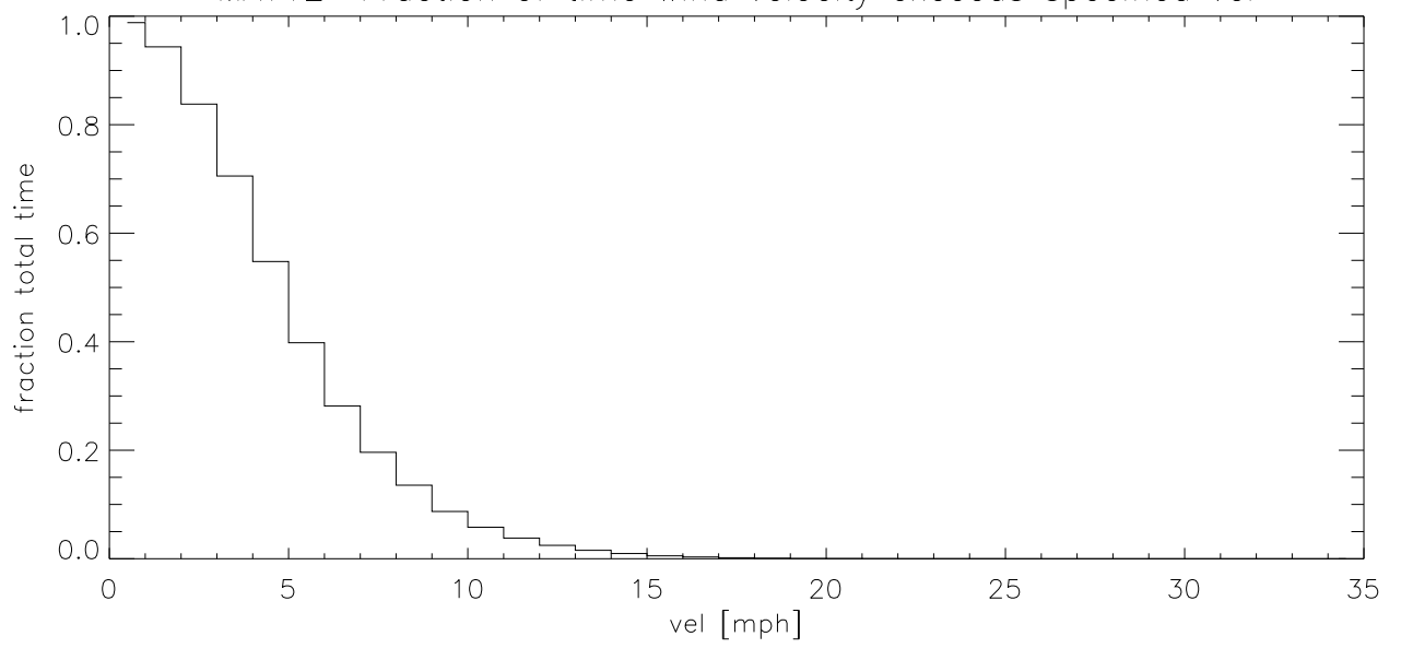
MAY12 Fraction of time wind velocity exceeds specified vel (blowup)
