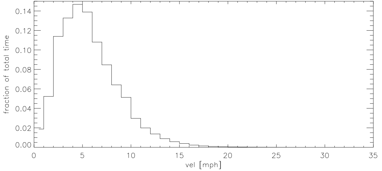
SEP11 Fraction of time wind velocity exceeds specified vel
