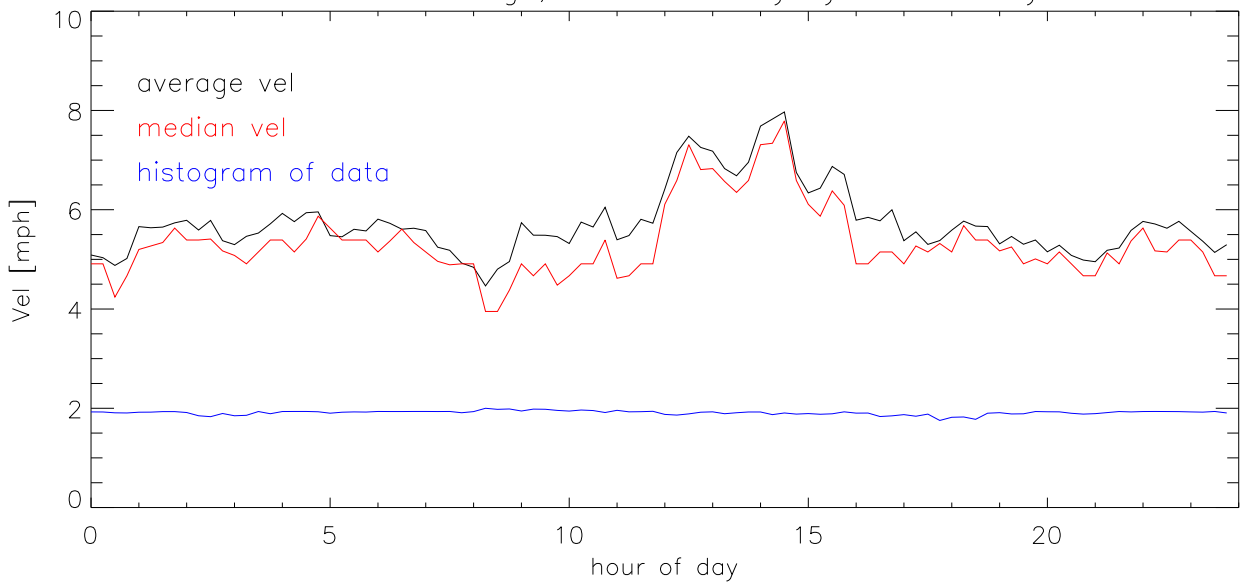
SEP11 Average,median velocity by direction
