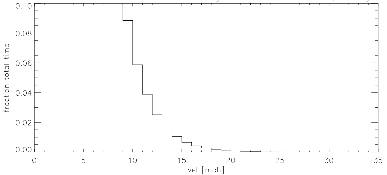
SEP11 Fraction of time wind velocity exceeds specified vel (blowup)
