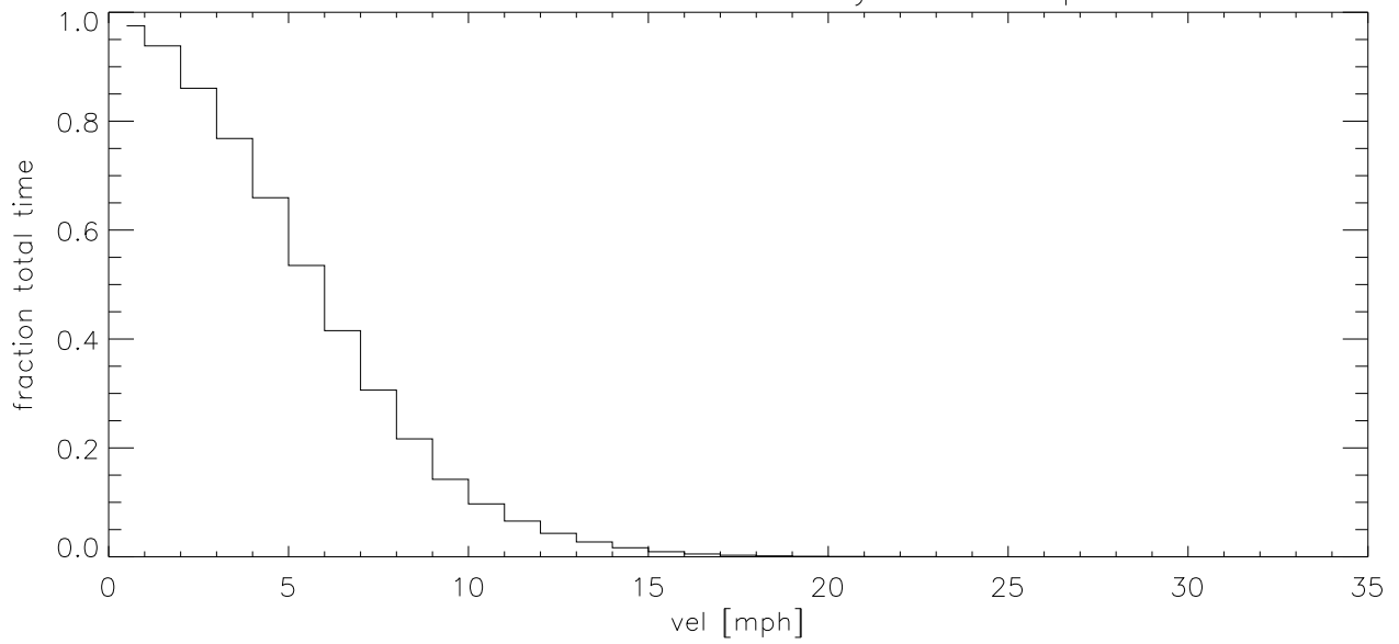
JUL11 Fraction of time wind velocity exceeds specified vel (blowup)
