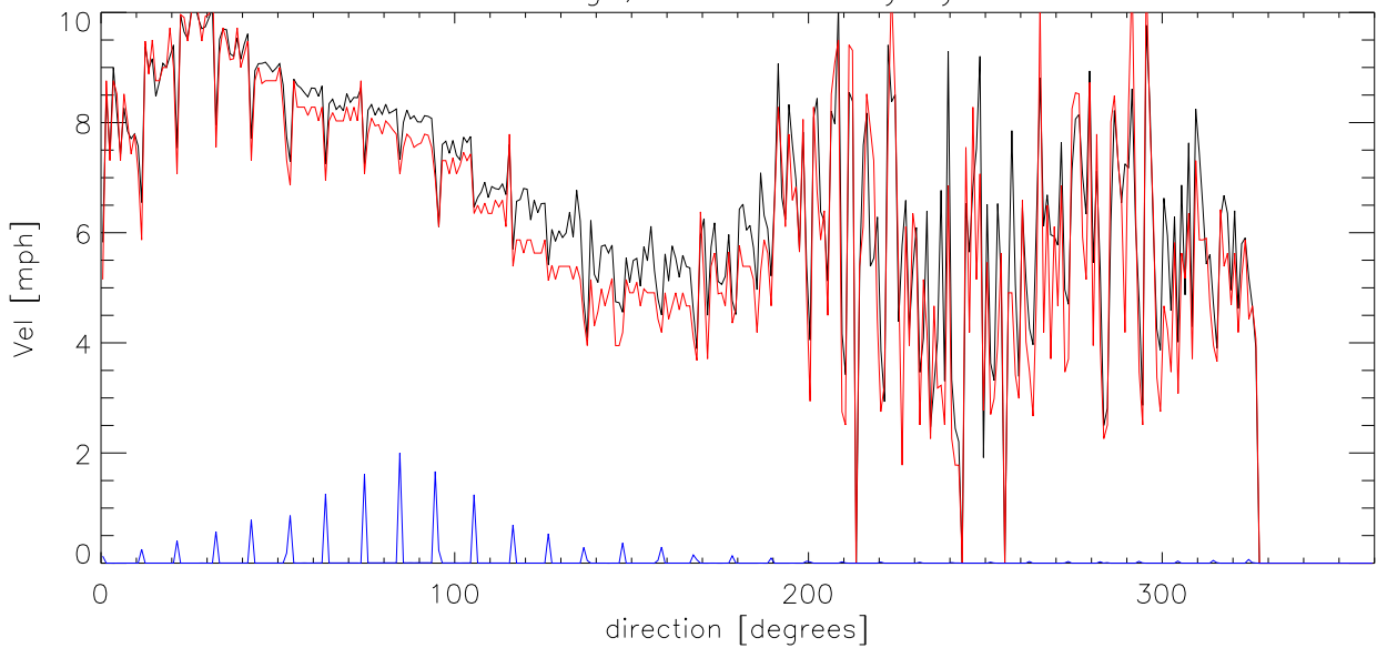
JUL11 Average, median velocity by direction
