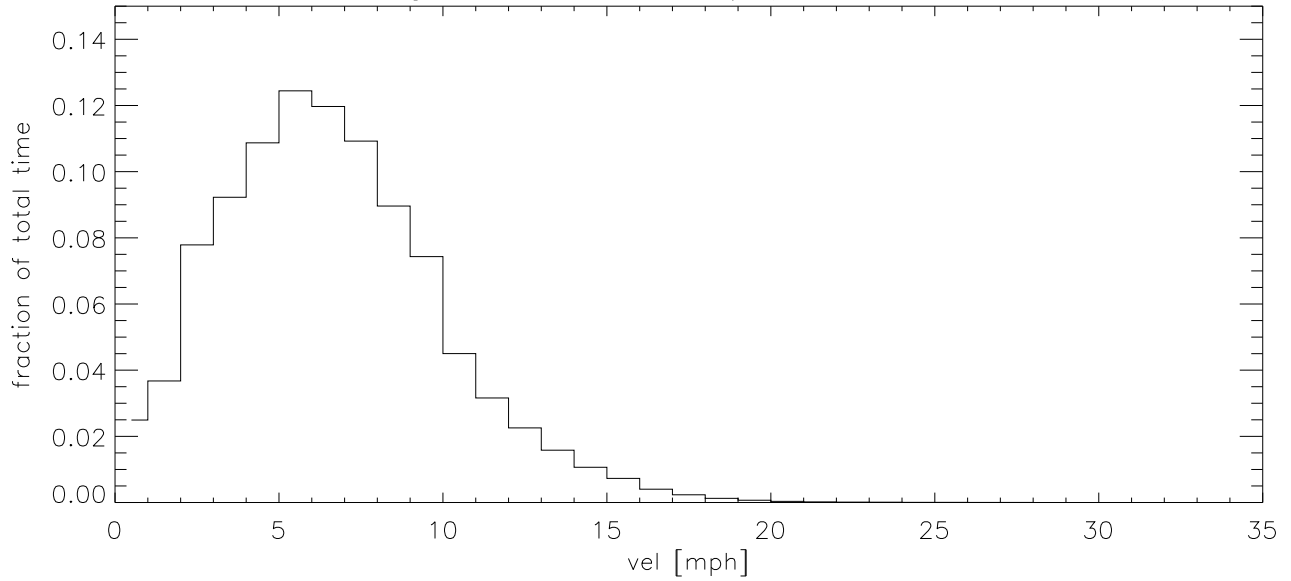
JUL11 Fraction of time wind velocity exceeds specified vel
