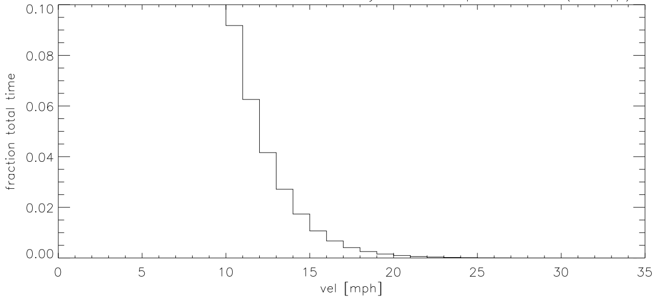
JUN11 Fraction of time wind velocity exceeds specified vel (blowup)
