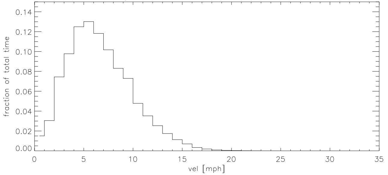
APR11 Fraction of time wind velocity exceeds specified vel
