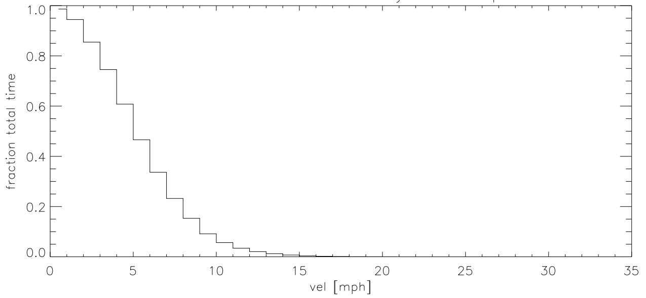
DEC10 Fraction of time wind velocity exceeds specified vel (blowup)
