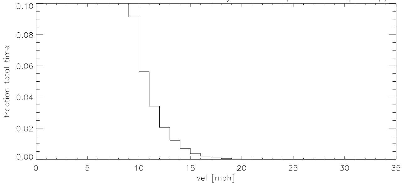
DEC10 Fraction of time wind velocity exceeds specified vel (blowup)
