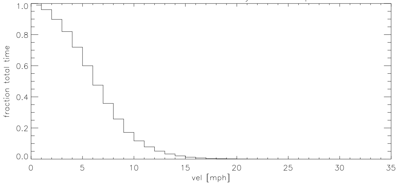
NOV10 Fraction of time wind velocity exceeds specified vel (blowup)
