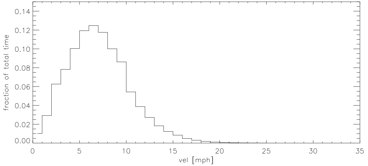
NOV10 Fraction of time wind velocity exceeds specified vel
