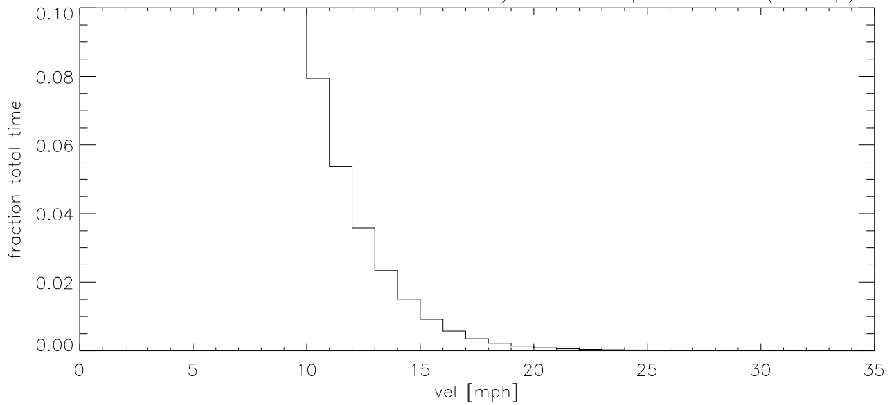
OCT10 Fraction of time wind velocity exceeds specified vel (blowup)
